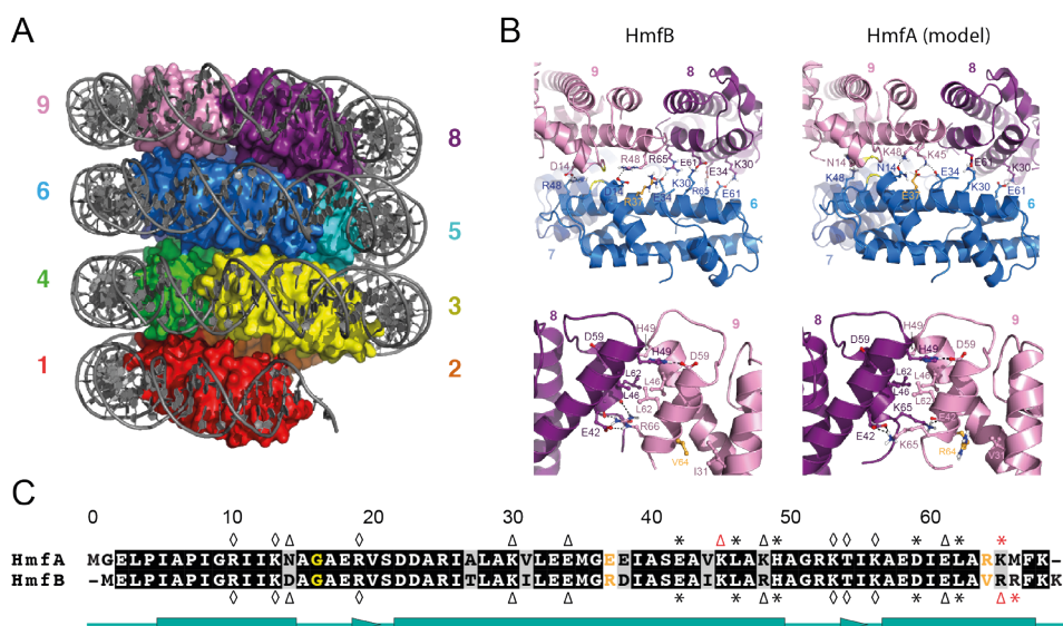
Figure 4.1: The hypernucleosome and Methanothermobacter fervidus histones HMfB and HMfA.
