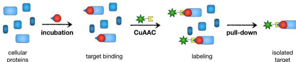
Scheme 1.4. Drug pull-down experiments allow for the identification of the drug binding partners. The drug (in red), functionalized with a handle (in blue), is incubated and labeled with a reporter tag (in green, here via CuAAC). This method allows for the separation of the metallated proteins. The isolated protein targets can be further analyzed and identified by MS.
