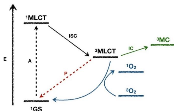
Scheme 1.2. Jablonski diagram of the photoactivation of d^6 transition metal complexes and their physical relaxation pathways in phototherapy. In the presence of molecular oxygen, photodynamic therapy (PDT) can lead to the production of reactive oxygen species (ROS) such as ^1\text{O}_2 (in blue). In photoactivated chemotherapy (PACT), population of the ^3\text{MC} state leads to ligand substitution (in green). Dashed lines indicate processes involving photons. Non-radiative decay from the ^3\text{MLCT} and ^3\text{MC} state are omitted for clarity. Abbreviations: A = absorption, ISC = Intersystem crossing, IC = internal conversion, P = phosphorescence.
