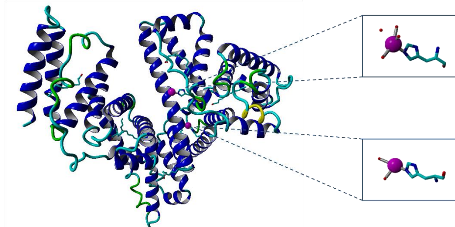
Figure 1.5. XRD structure of the KP1019-HSA adduct. All ligands are dissociated before binding of the ruthenium ion occurred at the histidine residues. 48
