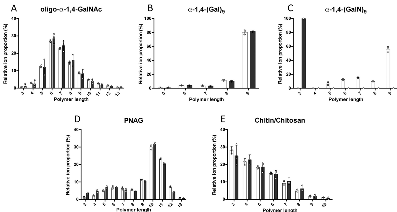
Figure 5. Ega3 is an endo- \alpha -1,4-galactosaminidase. MS analyses of oligosaccharide substrates before (white bars) and after treatment with 10 \mu M Ega3 for 24 h (black bars) are shown. Substrates include the following: A, purified oligo- \alpha -1,4-GalNAc isolated from GAG biofilms; B, synthesized \alpha -1,4-(Gal) 9 ; C, synthesized \alpha -1,4-(GalN) 9 ; D, synthesized oligo- \beta -1,6-GlcNAc (PNAG); and E, chitin/chitosan. Statistically significant differences between pre- and post-treatment oligosaccharide profiles were observed only for \alpha -1,4-(GalN) 9 in C.
