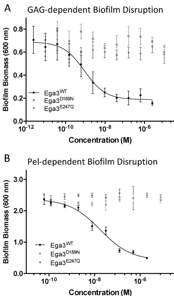
Figure 3. Ega3 treatment disrupts A. fumigatus and P. aeruginosa biofilm. Effects of the treatment with the indicated hydrolases on Af293 biofilms (A) and Pel-dependent P. aeruginosa PA14 biofilms (B). Residual biofilm biomass was quantified by crystal violet staining.
