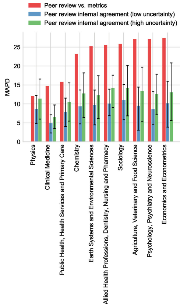
Fig. 5 Size-dependent median absolute percentage difference (MAPD) of P(\text{top } 10\%) relative to P(4^*) compared with the MAPD based on a model of peer review uncertainty. Results are shown only for the 10 units of assessment with the lowest MAPD of metrics relative to peer review
