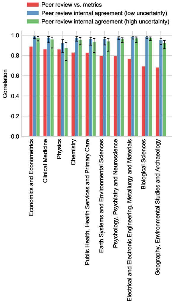
Fig. 2 Size-independent correlation between PP(top 10%) and PP(4 + ) compared with correlations based on a model of peer review uncertainty. Results are shown only for the 10 units of assessment with the highest correlation between metrics and peer review
