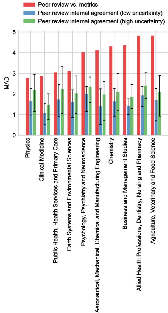
Fig. 3 Size-independent median absolute difference (MAD) between PP (top 10%) and PP(4 + ) compared with the MAD based on a model of peer review uncertainty. Results are shown only for the 10 units of assessment with the lowest MAD between metrics and peer review
