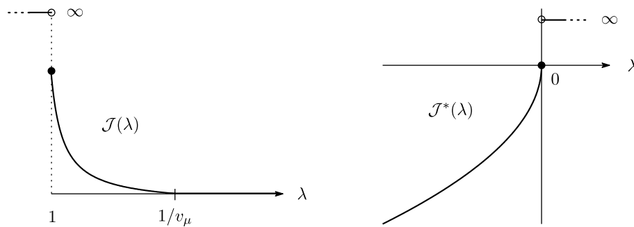
Figure 1: Left: Graph of \mathcal{J} , the quenched rate function of RWRE hitting times in (1.10). Right: Graph of \mathcal{J}^* , the scaled cumulant generating function of RWRE hitting times in (1.11).
