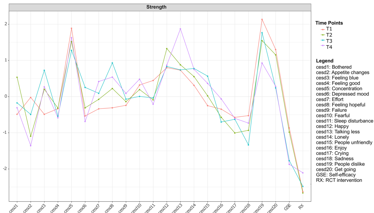
Fig 2. Centrality analysis of the 20 CES-D symptoms, self-efficacy (GSE) and intervention (RX).
