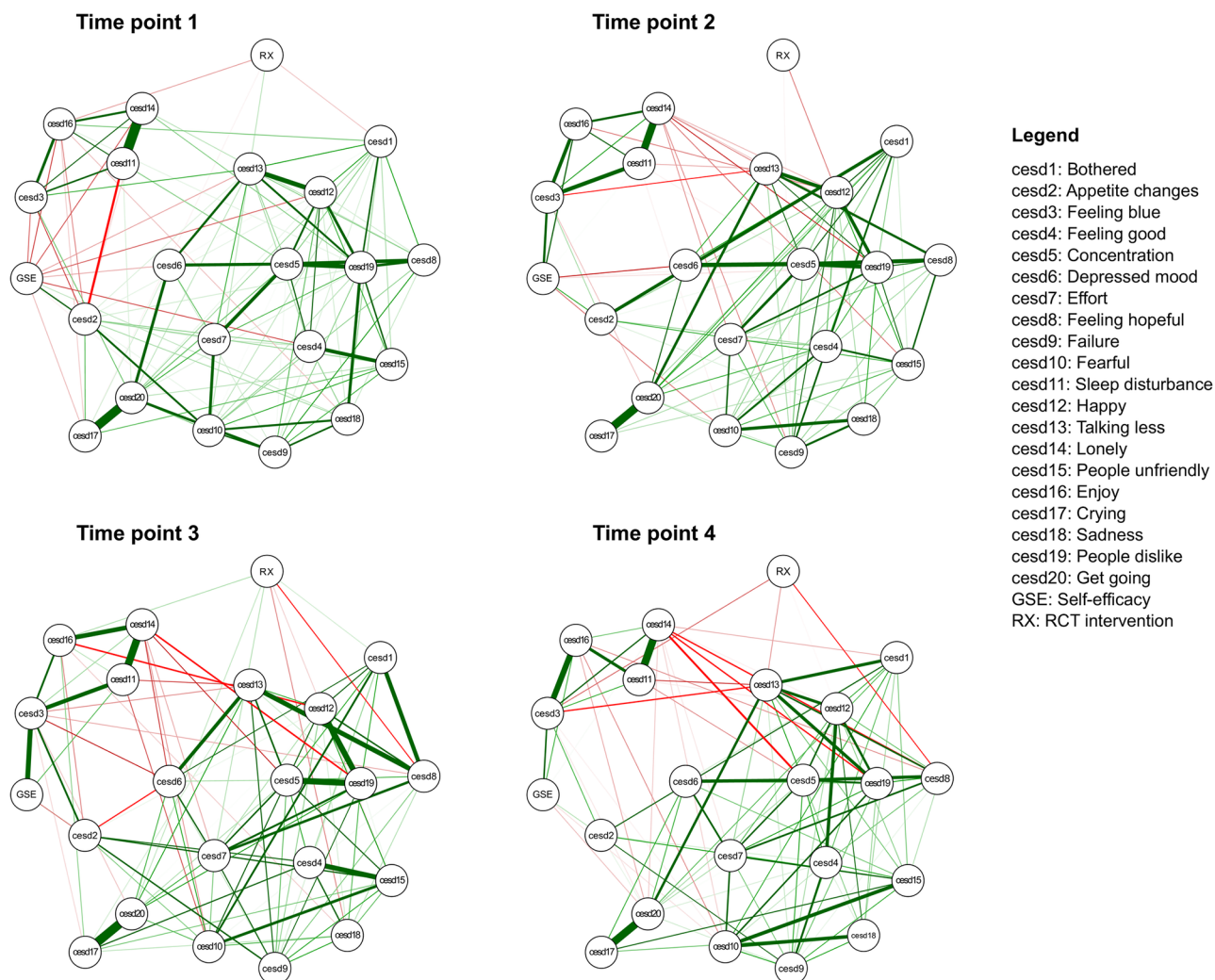
Fig 1. Network structure of the 20 CES-D symptoms, self-efficacy (GSE) and intervention (RX).
