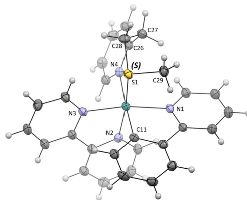
Figure 3. Displacement ellipsoid plot (50% probability level) of the \Lambda enantiomer of the cationic complex in the crystal structure of the pair \Lambda -(S)/ \Delta -(R)-ax-[4d]PF 6 at 110(2) K. The hexafluorophosphate counteranion has been omitted for clarity.
