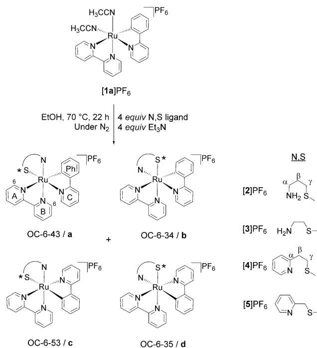
Scheme 1. Synthesis of [2] PF_6 , [3] PF_6 , [4] PF_6 , and [5] PF_6 from [1a] PF_6 and the structures of the four possible coordination isomers obtained. Note that, in order to obtain isomers c and d , the polypyridyl ligands must rearrange so the \sigma -bound C atom becomes trans to the entering N,S ligand. For clarity, only the \Delta isomers are shown, but all samples were obtained as racemic \Delta/\Lambda mixtures.
