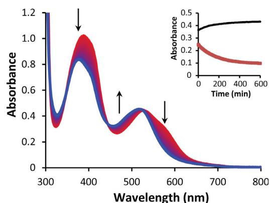
Figure 5. Evolution of the UV/Vis spectra of a solution of [4]PF 6 in CH 3 CN upon irradiation with a 521 nm LED (photon flux 6.80 \times 10^{-8} mol s -1 ) under N 2 . Inset: black dots represent the absorbance at 500 nm vs. time, and red squares represent the absorbance at 590 nm vs. time.
