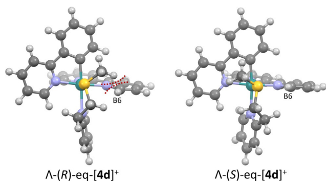
Figure 2. DFT structures of stereoisomers \Lambda -(R)-eq-[4d] + and \Lambda -(S)-eq-[4d] + . The isomer with the sulfur in R configuration (left) shows a very short distance between the methyl group and proton B6 on bipyridine, whereas in the isomer with the sulfur in S configuration the methyl group is much further from B6 and resides above the centre of the phpy - ligand, which lowers steric repulsion. This difference in steric interactions is observed in all computed R/S pairs.
