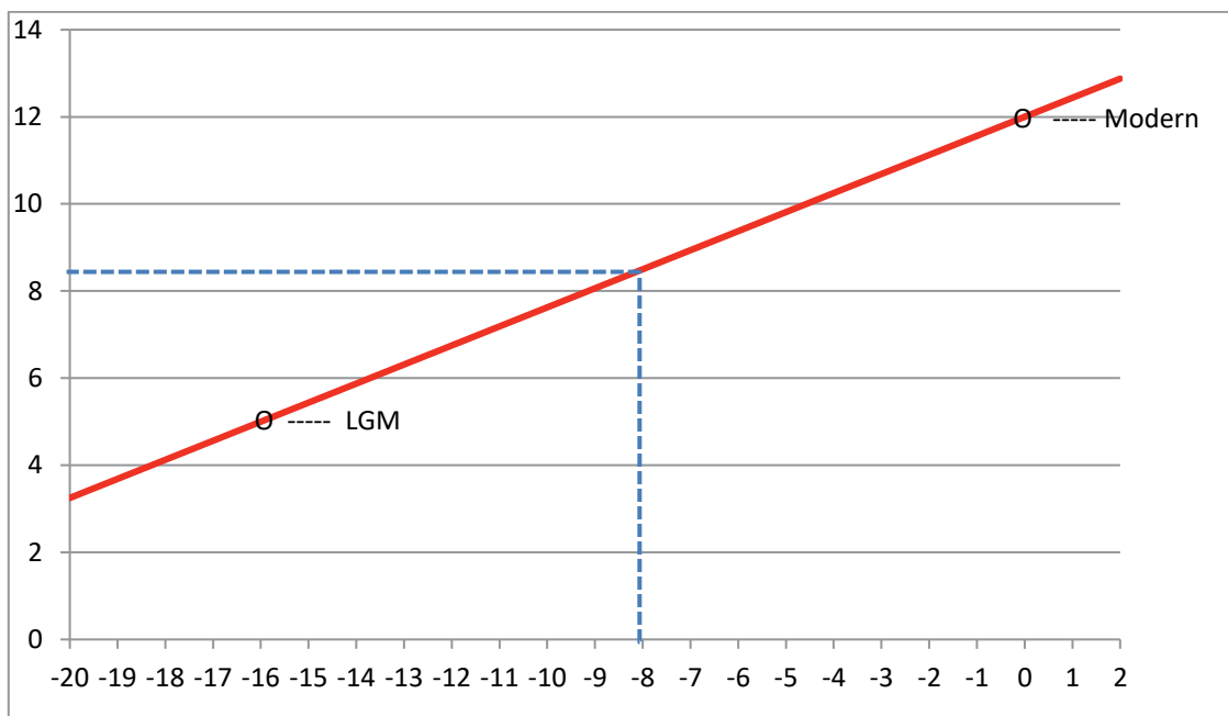
Figure 10: Interpolation of temperature values between two given data points: LGM and modern day values, with horizontally the reconstructed global mean temperature used as index for the linear interpolation.
