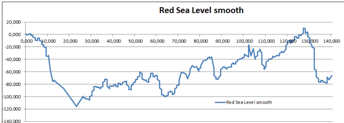
Figure 8: Red Sea level until 140 ka adapted from the supplementary materials from Grant et al. (2012) converted to equidistant horizontal axis.
