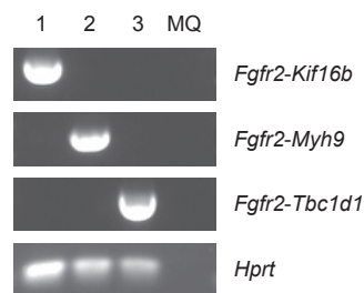
Fig. S4.7. Validation of endogenous Fgfr2 fusions from the ILC dataset via targeted PCR on cDNA. (A) Overview of endogenous fusions from STAR-Fusion (Supplementary Table S4.10) involving Fgfr2 , which reflect oncogenic fusions of FGFR2 identified in human breast cancers. (B) Validation results for these fusions, showing that each of the expected fusions is indeed detected in the cDNA of the corresponding sample. MQ (= MilliQ) is a water control, which was used as a negative control.
