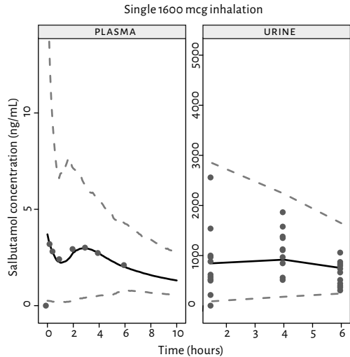
FIGURE 2 VISUAL PREDICTIVE CHECK OF SIMULATED CONCENTRATIONS AFTER AN INHALATION OF 1600 MCG SALBUTAMOL Black solid line: median predicted concentrations. Grey dashed lines: 95% concentration prediction interval. Grey points: observations extracted from Haase et al. 6 Left panel: plasma concentrations. Right panel: urine concentrations
