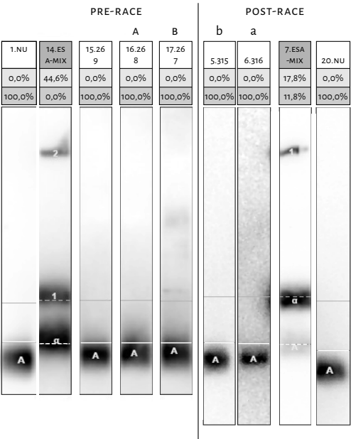
FIGURE 5 EXAMPLE OF CHANGES IN SARCOSYL-PAGE RESULTS DURING THE RACE Images of the sarcosyl-PAGE assay results taken from two gels. In lanes 16.268 and 17.267 urine samples taken pre-race from two subjects receiving rHuEPO were analysed. In lanes 5.315 and 6.316 samples taken post-race from the same subjects were analysed. Letters indicate the relevant lanes, with the A and a indicating lanes from one subject, and B and b from the other. Lanes labelled ESA-MIX are reference samples, lanes labelled NU are negative quality controls, the white line indicates the level where rHuEPO will stain. In lanes 16.268 and 17.267 staining is clearly present above the white line, while this is not the case in the samples from the same subjects that were taken only approximately 8 hours later, after the race, in lanes 5.315 and 6.316.
