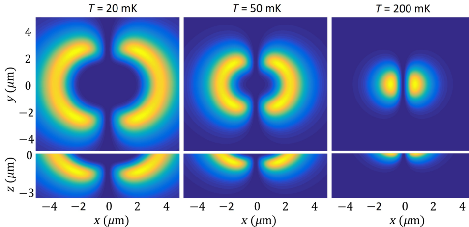
FIG. 6. Simulation of the relative contribution of spins at different locations, calculated for a tip-sample separation of 20 nm. Yellow indicates regions of maximal coupling, while blue indicates a very low coupling between a spin and the cantilever.
