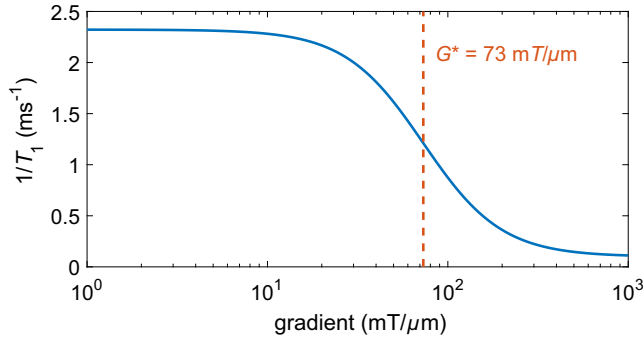
FIG. 5. Plot of the inverse of the T_1 time calculated from Eq. (11), using G^* = 73 \text{ mT}/\mu\text{m} , T_1^{\text{ff}} = 0.45 \text{ ms} , and T_1^* = 10 \text{ ms} .
