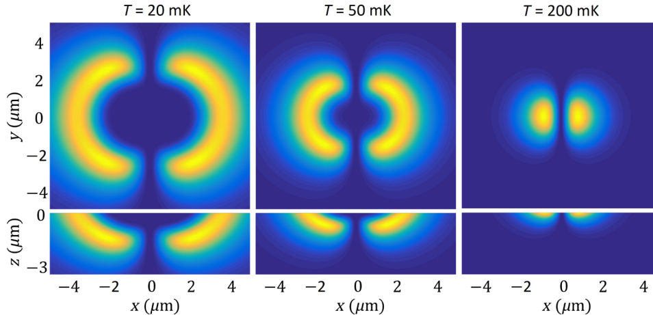
FIG. 6. Simulation of the relative contribution of spins at different locations, calculated for a tip-sample separation of 20 nm. Yellow indicates regions of maximal coupling, while blue indicates a very low coupling between a spin and the cantilever.
