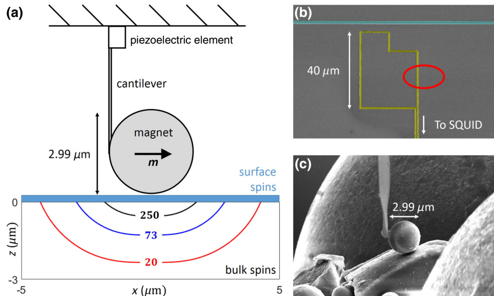
FIG. 1. (a) Setup: A magnetic particle with a diameter of 2.99 \text{ }\mu\text{m} attached to the end of a soft MRFM cantilever is positioned above the diamond sample, where it induces a high magnetic field gradient (solid colored lines, unit millitesla per micrometer). The bulk of the diamond contains nitrogen impurities with an associated electron spin. On the surface we find an impurity layer containing paramagnetic electron spins, indicated in blue. (b) False-color scanning-electron-microscope image of the nanofabricated structures on top of the diamond sample. The pickup loop used for the read-out of the cantilever is shown in yellow. In blue there is a niobium titanium nitride rf wire, which is not used in the current experiment. The measurements described in this work are done at the location marked by the red circle. (c) Scanning-electron-microscope image of the tip of the cantilever and a (Nd,Fe)B particle after the electron-beam-induced deposition.
