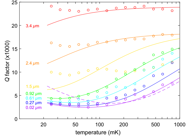
FIG. 4. Data (circles) and theory (lines) for the change in the quality factor of the cantilever versus temperature when the cantilever is positioned near the surface of the diamond sample. The solid lines are calculated with the spin densities obtained from the frequency data, including the effects of spin diffusion using T_1^* = 10 ms and T_1^{\text{ff}} = 0.45 ms. The dashed line shows the expected quality factor at a height of 0.02 \mu\text{m} calculated with a constant T_1 = 1.3 ms.
