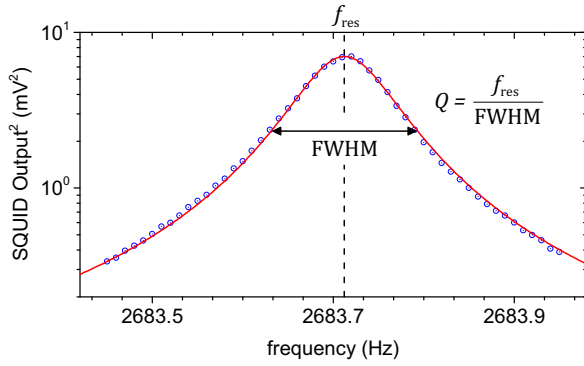
FIG. 2. Example of a frequency sweep measured at a tip-sample separation of 3.4 \mu\text{m} at a temperature of 25 mK. The resonance frequency and quality factor are obtained by the fitting of the data to a Lorentzian (solid red line).
