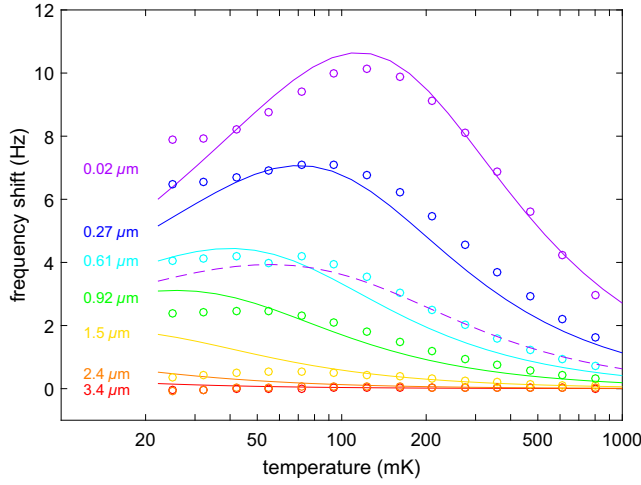
FIG. 3. Data (circles) and theory (lines) for the frequency shift of the cantilever versus temperature when the cantilever is positioned near the surface of the diamond sample. The dashed line shows the contribution from the bulk spins in the diamond only. The solid lines are calculated with \sigma = 0.072 spins/nm 2 and \rho = 0.40 ppm.
