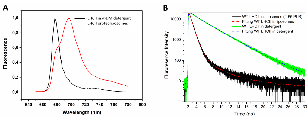
Figure 4. A: 77K fluorescence spectra of LHCII in \alpha -DM detergent (black) and after inserting into liposomes (red). B: time resolved fluorescence traces of LHCII in \alpha -DM detergent (green) and of LHCII in liposomes (black).
