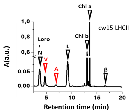
Figure 3. HPLC analysis of trimeric LHCII indicating the presence of violaxanthin.
