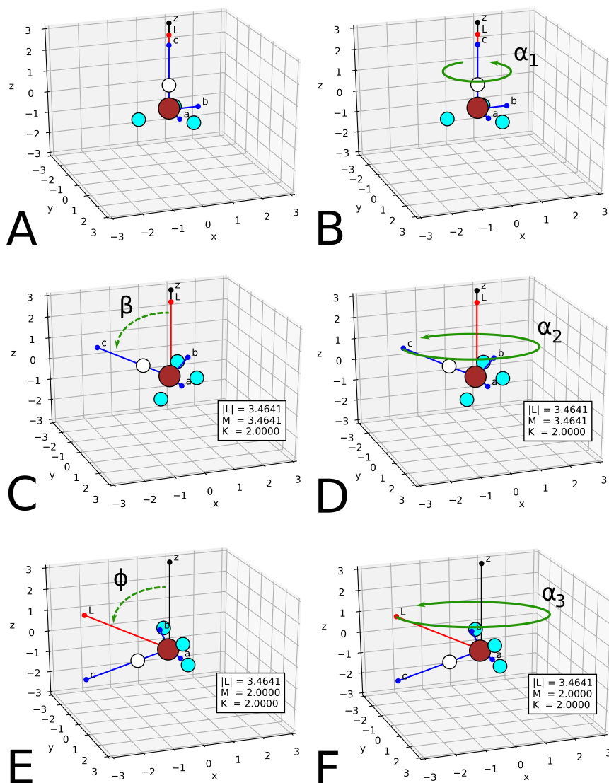
Figure 2.1: Scheme of the rotations needed to prepare the \text{CHD}_3 molecule in a generic aligned rotational state ( J = 3 , M = 2 , K = 2 ). The carbon atom is reported in brown, the hydrogen in white and the deuteriums in light blue. The reference frame axis z is reported in black and the molecular axes a , b and c are reported in blue. The angular momentum \mathbf{L} is indicated in red. Dashed green arrows indicate rotations to obtain the correct projections of \mathbf{L} and full green arrows indicate rotations that are sampled randomly. The values on the axes are reported in \text{\AA} and |\mathbf{L}| is in atomic units.
