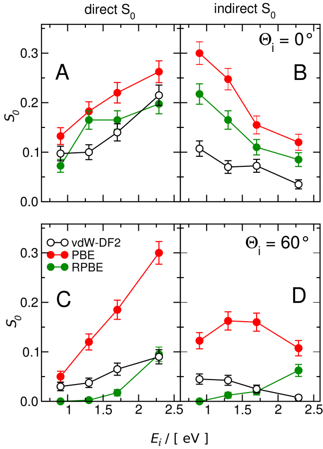
Figure 3.10: Direct (A, C) and indirect (B, D) reaction probability as a function of E_i for \Theta_i = 0^\circ (A, B) and \Theta_i = 60^\circ (C, D). vdW-DF2 results are reported as black empty circles. PBE and RPBE data (full red and green circles, respectively) for normal incidence are taken from Ref. [15].
