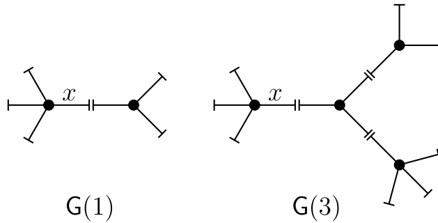
FIG. 6. Example snapshots of G(s) at times s = 1 and s = 3 .
