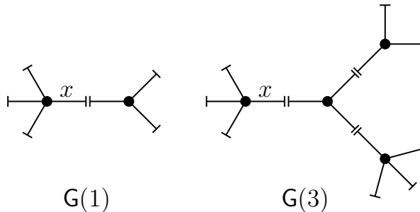
Figure 6: Example snapshots of G(s) at times s = 1 and s = 3 .
