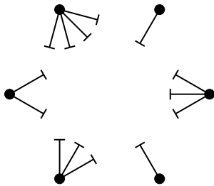
Figure 1: Vertices with half-edges.
