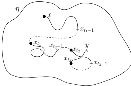
Figure 4: An example of a segmented path with 4 segments. Solid lines represent the segments, consisting of a path of half-edges in \eta , dashed lines indicate the succession of the segments. The latter do not necessarily correspond to a pair in \eta , and will later correspond to rewired edges in the graph dynamics.
