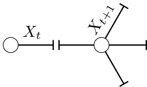
Figure 3: The random walk moves from half-edge X_t to half-edge X_{t+1} , one of the siblings of the half-edge that X_t is paired to.
