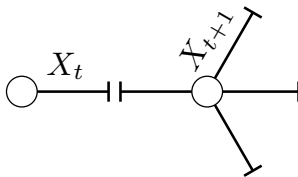
Figure 3: The random walk moves from half-edge X_t to half-edge X_{t+1} , one of the siblings of the half-edge that X_t is paired to.
