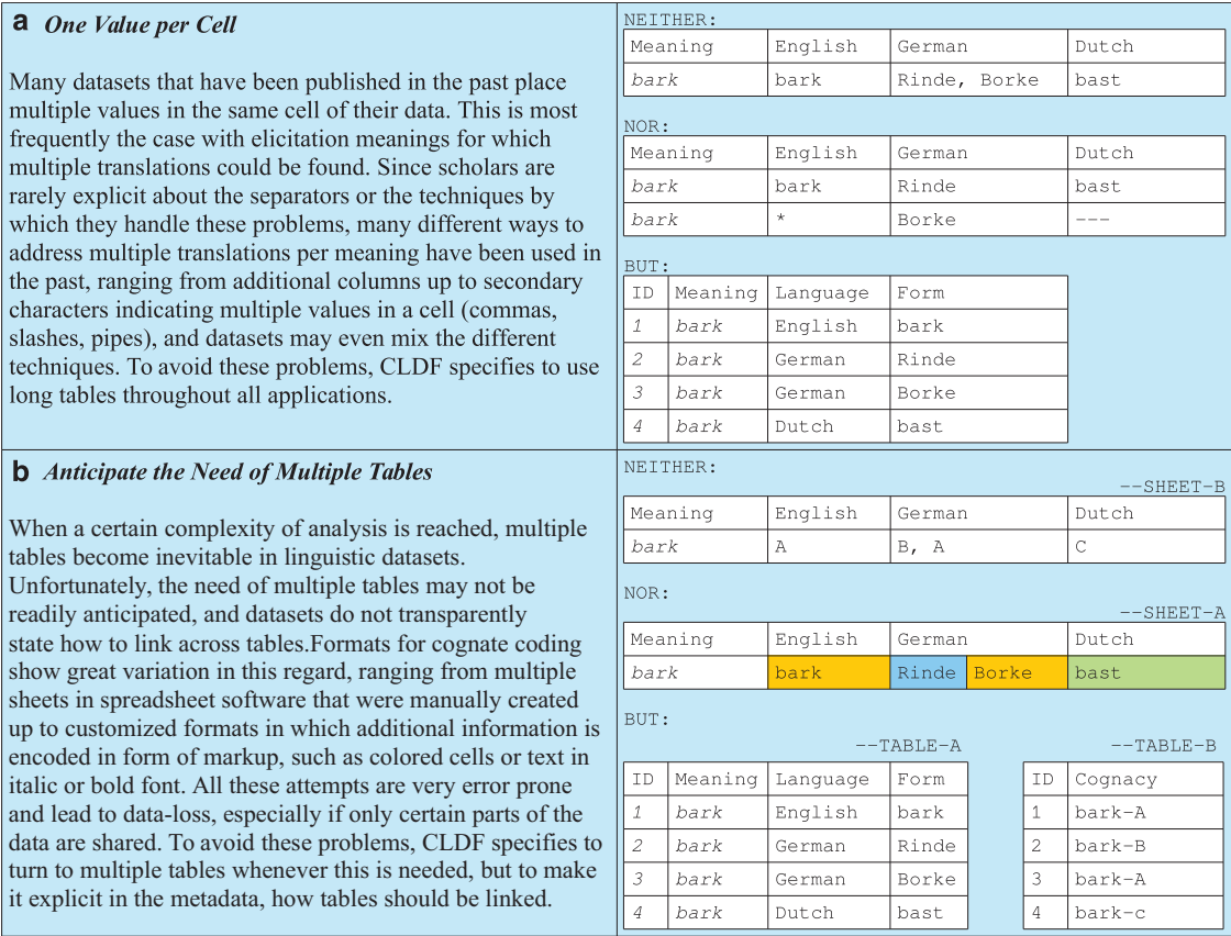
Figure 1. Basic rules of data coding, taking cognate coding in wordlists as an example. (a) Illustrates why long tables 53 should be favored throughout all applications. (b) Underlines the importance of anticipating multiple tables along with metadata indicating how they should be linked 44 .
