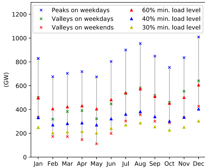
Fig. 8. Illustration of positions of average peaks, valleys and minimum load in each month in S2.
