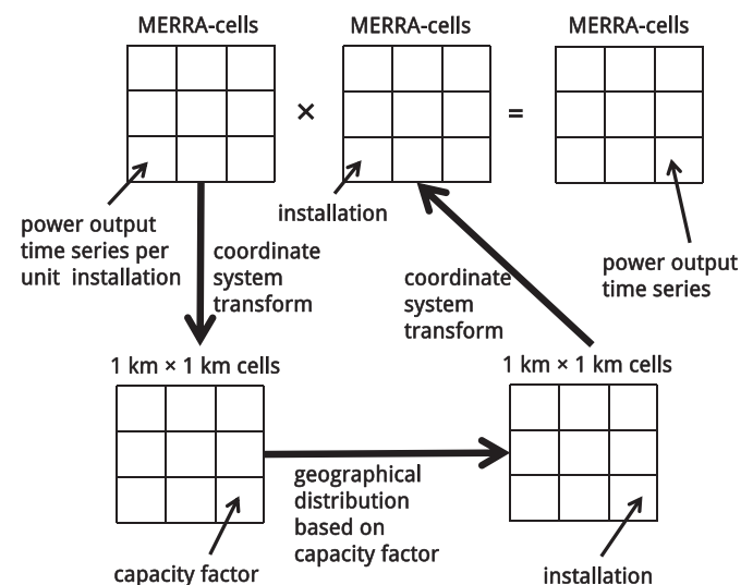
Fig. 1. Calculation of VREs generation time series in each MERRA-cell.
