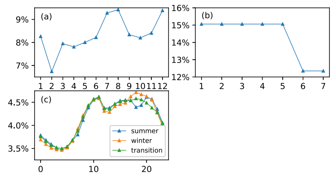
Fig. 4. Normalized monthly (a), weekly (b) and daily (c) load curves.
