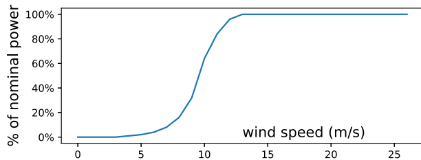
Fig. 2. Wind power curve (cut-in speed: 3 m/s, cut-off speed: 25 m/s, rated speed: 11 m/s).
