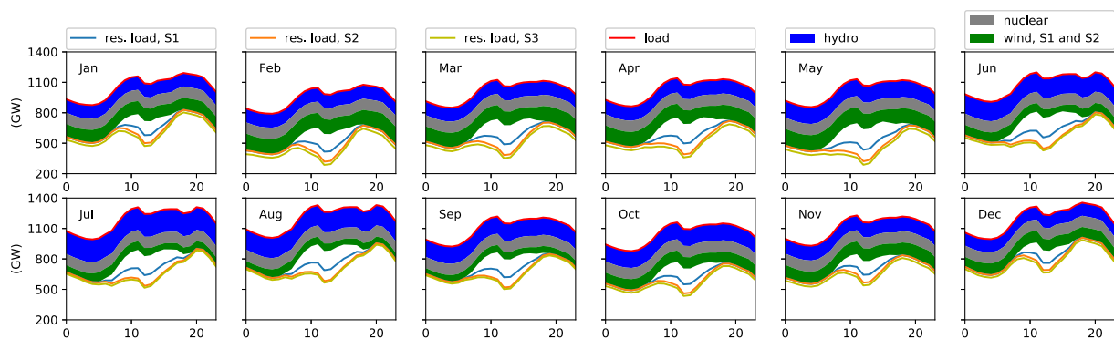
Fig. 6. Average daily shapes of load and residual load in S1, S2 and S3 on weekdays, and average daily generation of hydropower, nuclear power and wind power. Hydropower and nuclear power are the same in S1, S2 and S3. Wind generation in S1 and S2 are shown in the green area. Note that in our scenarios setting, S2 has 3% more PV power than S1, and S3 has 3% more wind power than S2. The area between blue line and orange line is the 3% PV power, the area between orange line and yellow line is the 3% wind power. (For interpretation of the references to colour in this figure legend, the reader is referred to the Web version of this article.)
