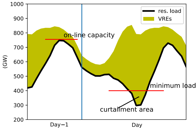
Fig. 5. Illustration of residual load and VREs generation in two consecutive days. Thermal power changes between its on-line capacity and minimum load, where on-line capacity is the sum of capacities of all active thermal power plants and minimum load = on-line capacity \times minimum load level. We assume that the VREs below the minimum load of on-line thermal power plants are curtailed.
