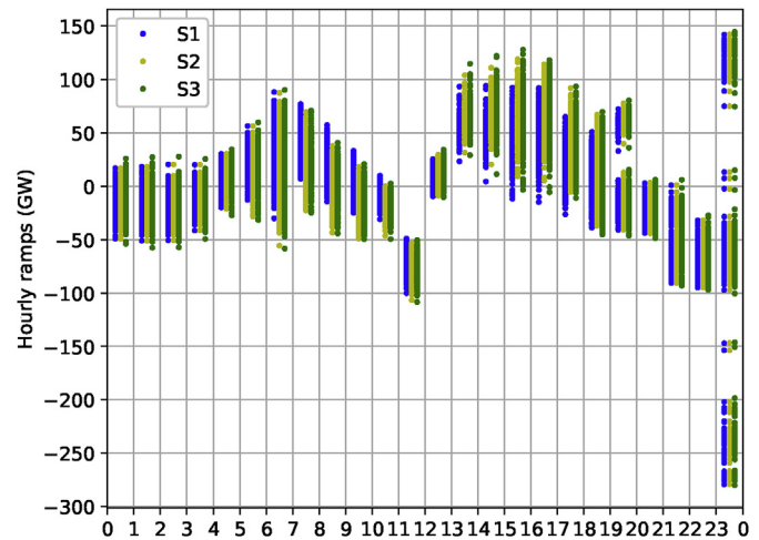
Fig. 7. Distributions of hourly ramps in 24 h.
