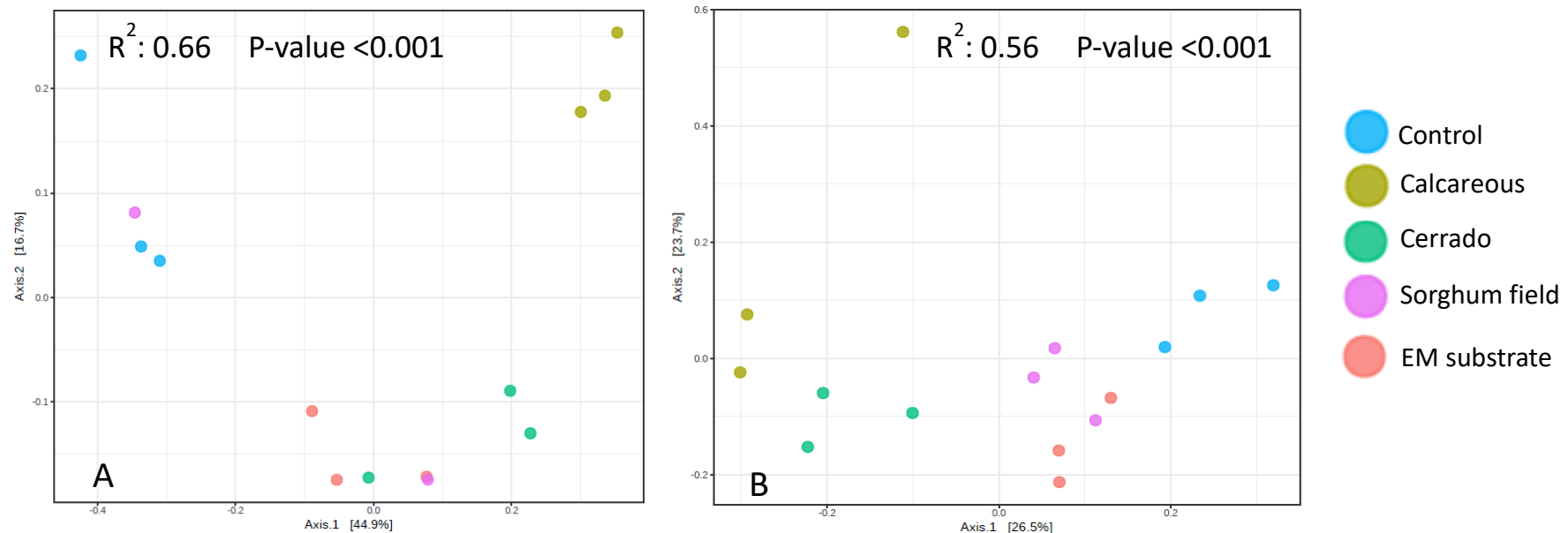
Figure 4. Principal Coordinate Analysis (PCoA) representing the dissimilarities of bacterial communities of two sorghum lineages (A) drought susceptible “9618158” and (B) drought tolerant “9910032” grown on different soils (Control, Calcareous, Cerrado, Sorghum field, and Enriched microbial – EM substrate) for 21 days and later transplanted to a standardized mixed substrate of sterilized sand and vermiculite (2:1 v/v). The rhizoplane bacterial community was sampled after grown for 38 days at standardized substrate at water deficiency moisture conditions.
