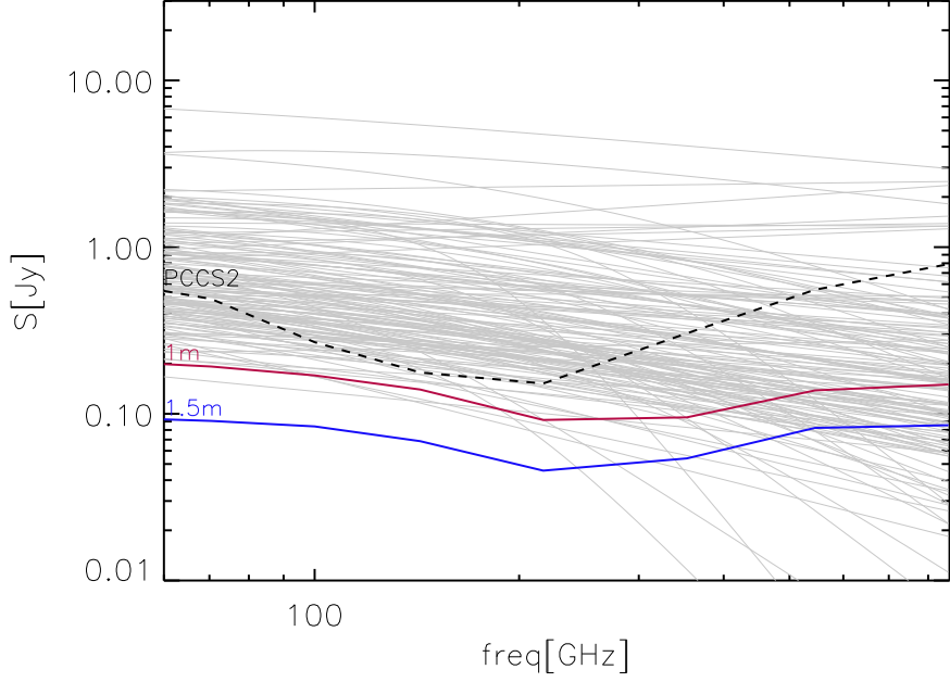
Figure 7. Continuum spectra of PACO-bright sources compared with the 90% completeness limits of the Planck /PCCS2 catalogue (dashed black line) and with the 4\sigma detection limits for the CORE 1-m (CORE100) and 1.5-m (CORE150) telescope sizes (solid red and blue lines, respectively). Note that, particularly at the highest frequencies, the fraction of PACO-bright sources whose fitted spectra are above the Planck /PCCS2 90% completeness limits is substantially larger than the number of actual Planck /PCCS2 detections, listed in Table 2; this may suggest that the fits over-predict the flux densities at frequencies beyond the highest frequency detections or that the PCCS2 completeness level is somewhat overestimated.
