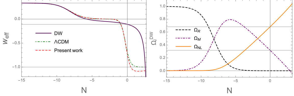
Figure 6. Left panel: Evolution of the effective equation of state w_{\text{eff}} as a function of the number of e -folds N for the DW \alpha R^{\frac{1}{2}}R model (black, solid curve), as well as for the model presented in this paper (red, dashed curve) and \Lambda CDM (green, dot-dashed curve). Right panel: Evolution of the density parameters \Omega_R (black, dashed curve), \Omega_M (violet, dot-dashed curve), and \Omega_{\text{NL}} (orange, solid curve) as functions of the number of e -folds N for the DW \alpha R^{\frac{1}{2}}R model. The lower and upper, grey, horizontal lines represent \Omega_M^0 and 1 - \Omega_M^0 - \Omega_R^0 , respectively.
