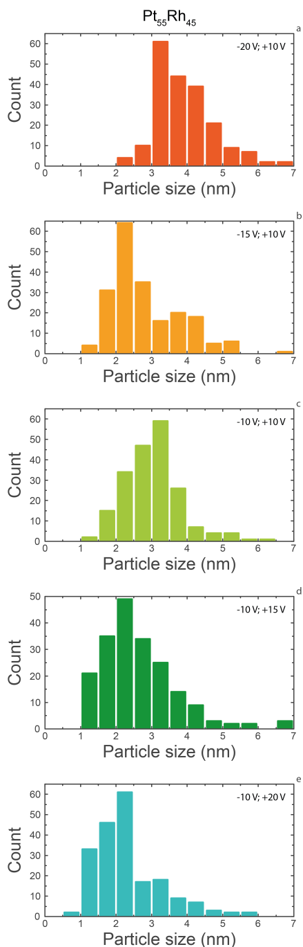
Fig. D.5 | Particle size distributions for studied \text{Pt}_{55}\text{Rh}_{45} nanoparticles.
