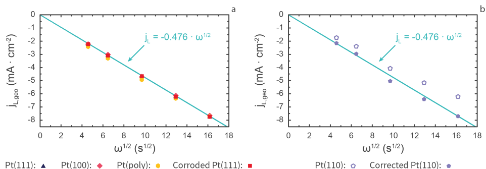
Fig. C.4 | Levich plots for the ORR on Pt(111), Pt(100), Pt(poly) and Pt(111) which was corroded at -1.0 V vs. RHE in 1 M NaOH (a) . Corrected and uncorrected Levich plots for the ORR on Pt(110) (b) . Voltammograms for acquiring the plotted datapoints were recorded in 0.1 M HClO 4 , at a scan rate of 50 mV · s -1 .
