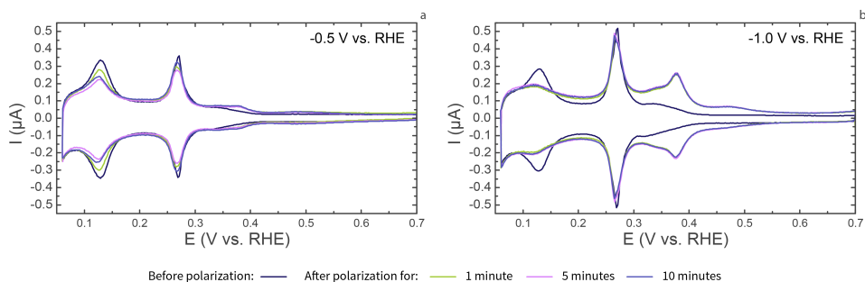
Fig. A.32 | CVs of platinum electrodes before (dark blue trace) and after cathodic polarization in 5 M NaOH at -0.5 V vs. RHE (a) and -1.0 V vs. RHE (b) for 1, 5 and 10 minutes. CV electrolyte: 0.5 M \text{H}_2\text{SO}_4 . Scan rate: 50 \text{ mV} \cdot \text{s}^{-1} .
