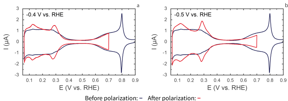
Fig. C.6 | Cyclic voltammograms of Pt(111) before (blue trace) and after (red trace) cathodic polarization in 10 M NaOH at -0.4 V vs. RHE (a) and -0.5 V vs. RHE (b) . Voltammograms were recorded in 0.1 M HClO 4 , at a scan rate of 50 \text{ mV} \cdot \text{s}^{-1} .
