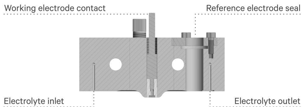
SIDE SECTION
