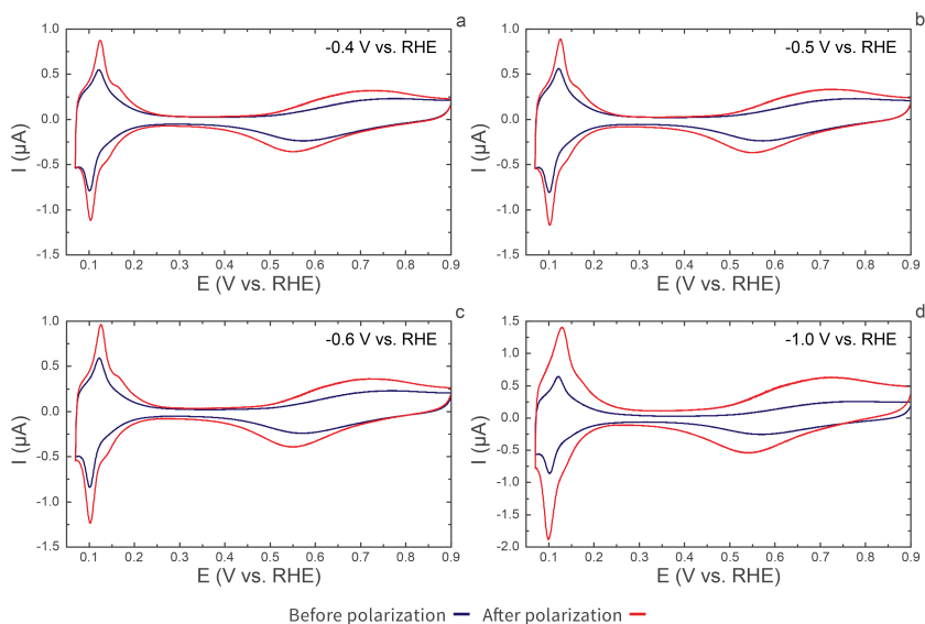
Fig. A.10 | CVs of Rh before (blue trace) and after (red trace) polarization in 5 M LiOH at -0.4 V vs. RHE (a) , -0.5 V vs. RHE (b) , -0.6 V vs. RHE (c) and -1.0 V vs. RHE (d) . CV electrolyte: 0.1 M \text{H}_2\text{SO}_4 . Scan rate: 50 \text{ mV} \cdot \text{s}^{-1} .
