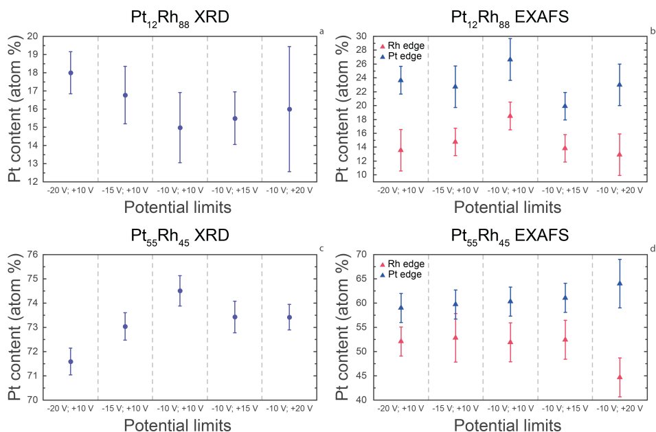
Fig. 7.4 | : Composition of nanoparticles produced from Pt 12 Rh 88 (a, b) and Pt 55 Rh 45 (c, d) wires, as determined by XRD (a, c) and EXAFS (b, d). Error bars represent one standard deviation.
