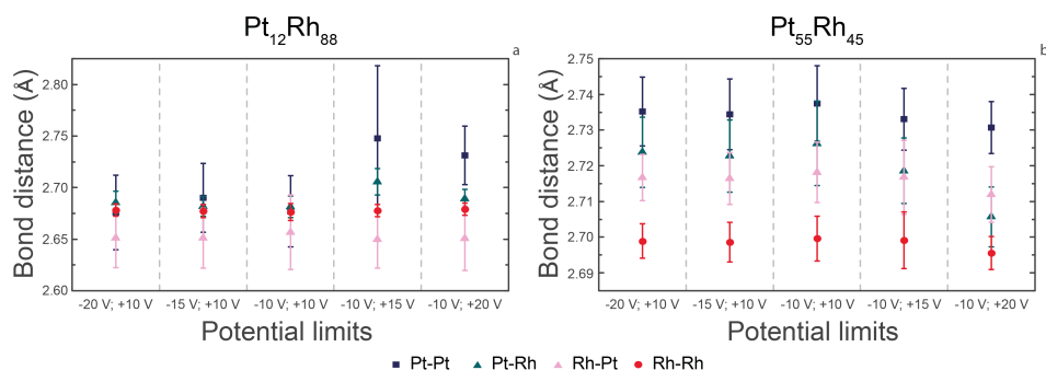
Fig. 7.6 | Average bond distances of Pt and Rh in Pt 12 Rh 88 (a) and Pt 55 Rh 45 (b). The Pt-Rh and Rh-Pt distances both represent the same distance, measured on a different absorption edge. The Pt-Rh data points were measured on the Pt L III edge, while the Rh-Pt points were measured on the Rh K edge. Error bars represent one standard deviation.
