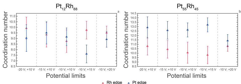
Fig. 7.5 | Average coordination numbers of Pt and Rh in Pt 12 Rh 88 (a) and Pt 55 Rh 45 (b). Error bars represent one standard deviation.
