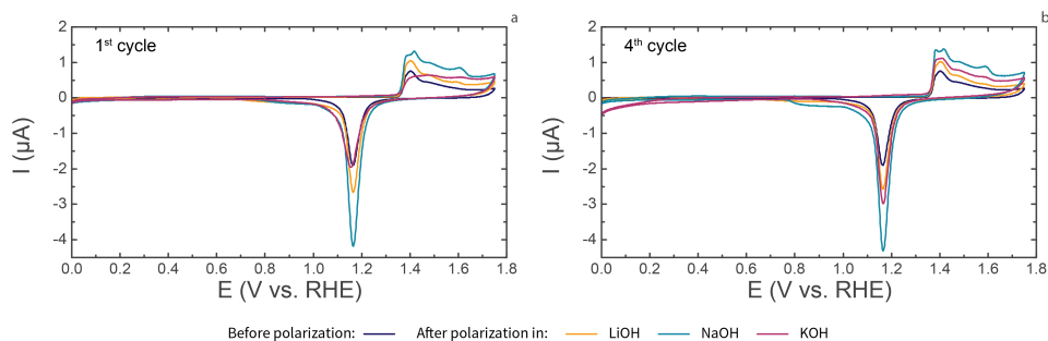
Fig. 4.7 | Cyclic voltammograms of Au, corroded in 5 M LiOH, 5 M NaOH and 5 M KOH at -1.5 V vs. RHE. CVs shown are the first cycle (a) and the fourth cycle (b) after cathodic corrosion. Voltammograms were recorded in 0.1 M \text{H}_2\text{SO}_4 , at a scan rate of 50 \text{ mV} \cdot \text{s}^{-1} .
