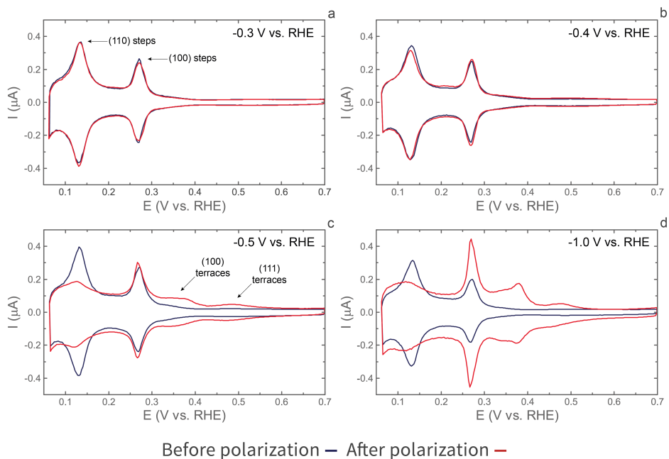
Fig. 2.1 | Cyclic voltammograms of platinum electrodes before (blue trace) and after (red trace) cathodic polarization in 10 M NaOH at -0.3 V vs. RHE (a) , -0.4 V vs. RHE (b) , -0.5 V vs. RHE (c) and -1.0 V vs. RHE (d) . Voltammograms were recorded in 0.5 M \text{H}_2\text{SO}_4 , at a scan rate of 50 \text{ mV} \cdot \text{s}^{-1} .
