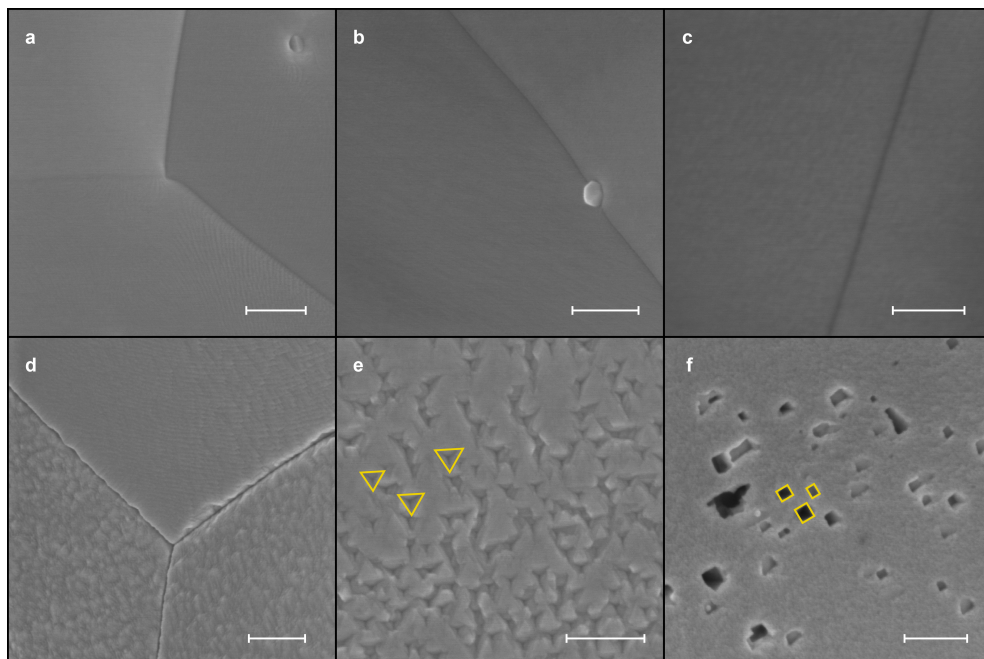
Fig. 2.2 | Scanning electron micrographs of platinum electrodes treated at -0.2 V vs. RHE ( a ), -0.4 V vs. RHE ( b ); -0.5 V vs. RHE ( c ); -0.6 V vs. RHE ( d, e ) and -0.8 V vs. RHE ( f ). In e, f , three etch pits have been outlined in yellow to illustrate shape and orientation similarities. Scale bars are 300 nm ( a, b, d-f ). Scale bar is 100 nm in Panel c .
