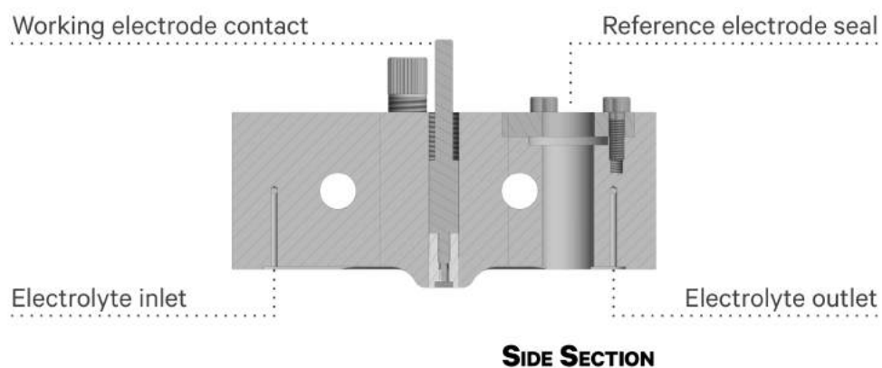
Fig. B.2 | Various schematic views of the employed flow cell. Aluminum cover plate is not shown in Perspective and Side Section.
