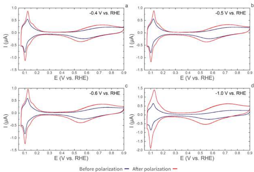
Fig. A.10 | CVs of Rh before (blue trace) and after (red trace) polarization in 5 M LiOH at -0.4 V vs. RHE (a), -0.5 V vs. RHE (b), -0.6 V vs. RHE (c) and -1.0 V vs. RHE (d). CV electrolyte: 0.1 M H 2 SO 4 . Scan rate: 50 mV · s -1 .
