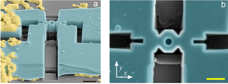
Figure 7.3: Falsed-color scanning electron microscope image of the ring yy146. a blue and yellow, respectively, represent the \text{Sr}_2\text{RuO}_4 crystal and the silver epoxy used for making electrical contact. The ring is connected to four transport leads, and is sculpted out of a 0.7 \mu\text{m} thick crystal by a \text{Ga}^+ focused ion beam. The surface of the crystal is protected by a 100 \text{ nm} \text{SiO}_x layer. b , close-up of the ring. The outer radius is 1.1 \mu\text{m} , and the inner radius is at least 0.2 \mu\text{m} . The dark and yellow scale bars correspond to 2 \mu\text{m} and 1 \mu\text{m} , respectively.
