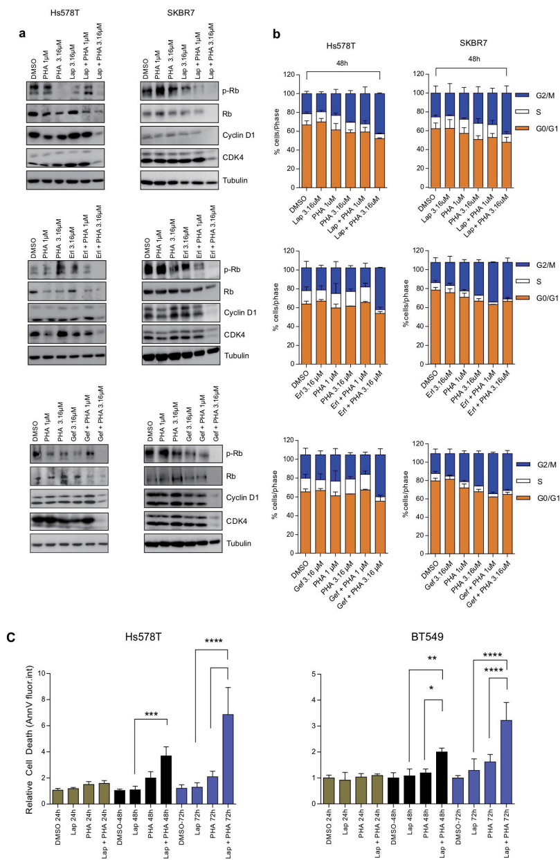
Figure 4: EGFR-TKIs and PHA-767491 synergise to induce G2/M cell cycle arrest and apoptosis. a. Inhibition of cell cycle components by co-treatment with EGFR-TKIs (lapatinib, erlotinib or gefitinib) and PHA-767491. Hs578T and SKBR7 cells were treated with EGFR-TKI alone (3.16 \mu M) or combined with PHA-767491 (1 \mu M or 3.16 \mu M) for 48 hours as indicated. b. Cell cycle distribution of Hs578T and SKBR7 cells after 48h treatment with EGFR-TKIs (3.16 \mu M) alone or combined with PHA-767491 (1 \mu M or 3.16 \mu M), as indicated. Data shown as mean of two independent experiments \pm standard deviation. c. Induction of apoptosis by EGFR-TKI and PHA-767491 co-treatment. Hs578T and BT549 cells were treated with lapatinib (3.16 \mu M), PHA-767491 (3.16 \mu M), alone or combined, as indicated, for 24h, 48h or 72h, respectively, and then stained with Annexin-V and Hoechst, followed by imaging and image quantification. Data shown as mean \pm standard deviation of two independent experiments. Relative cell death was quantified by normalising the intensity of Annexin-V signal to that of DMSO control. One-way ANOVA **** P \leq 0.0001 , *** P \leq 0.001 , ** P \leq 0.01 , * P \leq 0.05 .
