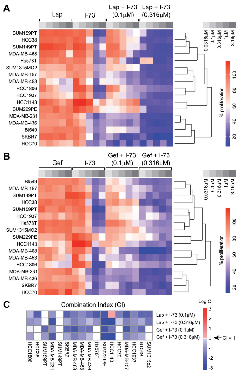
Figure 3. CDK9 inhibitor I-73 reverses the resistance of TNBC cells to EGFR-tyrosine kinase inhibitors. A. Effect of EGFR-TKI lapatinib (Lap) in concentration range combined with I-73 (0.1 \mu M or 0.316 \mu M) on the proliferation of TNBC cell lines. B. Effect of EGFR-TKI gefitinib (Gef) in concentration range combined with I-73 (0.1 \mu M or 0.316 \mu M) on the proliferation of TNBC cell lines. Data shown as percentage proliferation normalised to DMSO control. C. Synergistic CI evaluation of Lap + I-73 and Gef + I-73 combinations. Data shown as Log CI values. CI > 1, antagonism; CI = 1, additivity; CI < 1, synergy.
