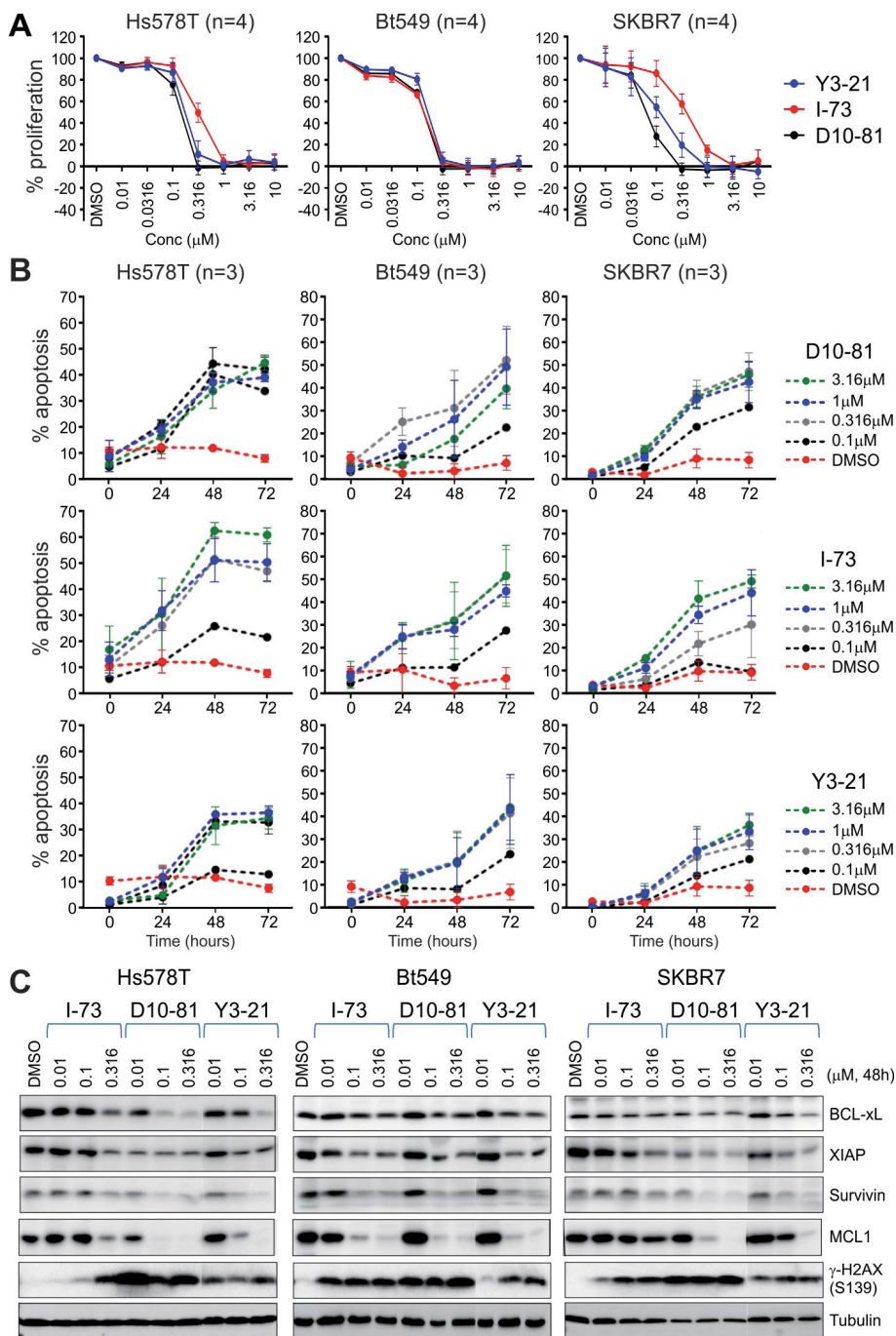
Figure 4. CDK9 inhibitors induce apoptosis in TNBC cells. (A) Validation of the anti-proliferative effects of the CDK9 inhibitors D10-81, I-73 and Y3-21 in selected TNBC cell lines Hs578T, BT549 and SKBR7. Data represented as mean \pm standard deviation (n = 4). (B) Apoptosis induction by the CDK9 inhibitors in TNBC cell lines Hs578T, BT549 and SKBR7. Cells were exposed to a dose range of each inhibitor (0.1-3.16 μM), and stained with Annexin-V and Hoechst as described for imaging at 24 hours, 48 hours and 72 hours post-exposure to CDK inhibitors or vehicle control (DMSO). Data were shown as % Annexin-V-positive cells, represented as mean \pm standard deviation (n = 3). (C) Impact of I-73, D10-81 and Y3-21 in dose range (0.01, 0.1 or 0.316 μM) on the inhibition of anti-apoptotic factors and the induction of DNA damage in representative Hs578T, BT549 and SKBR7 cells, 48 hours post-treatment.
