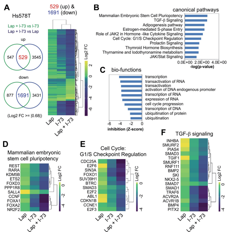
Figure 5. I-73 and lapatinib co-treatment disrupts the transcriptomic profile of TNBC cells. TNBC Hs578T cells were treated for 6 hours with Lap (3.16 \mu M), I-73 (0.1 \mu M), combined Lap + I-73 at the same doses, or DMSO as control, and harvested for RNA purification and RNA-Sequencing. Gene expression levels were presented in Log2 fold change (Log2 FC) normalized to control DMSO. A. Venn diagram and clustering of 529 up- and 1691 down-regulated genes in I-73 and lapatinib combination. Expression levels of genes under Lap + I-73 combined treatment were compared to those under single treatment Lap (Lap + I-73 vs Lap) or I-73 (Lap + I-73 vs I-73). Genes that overlapped in both comparisons and which were significantly up- (Log2 FC \geq +0.68) or down-regulated (Log2 FC \leq -0.68), were selected as synergy-related genes. The differential expression signature is shown in the heatmap. B. Top canonical pathways in which the Lap + I-73 synergy-regulated and differentially expressed genes are enriched, revealed by Ingenuity Pathway Analysis® (IPA). Significance was presented as -log p(value). C. Enrichment of Lap + I-73 synergy-related genes in top biological functions. Inhibitory effect was presented as Z-score. D. Expression of Lap + I-73 synergy-sensitive factors regulating mammalian embryonic stem cell pluripotency. E. Regulators of G1/S cell cycle in response to Lap + I-73 synergy. F. Sensitivity of TGF- \beta pathway members to Lap + I-73 synergy.
