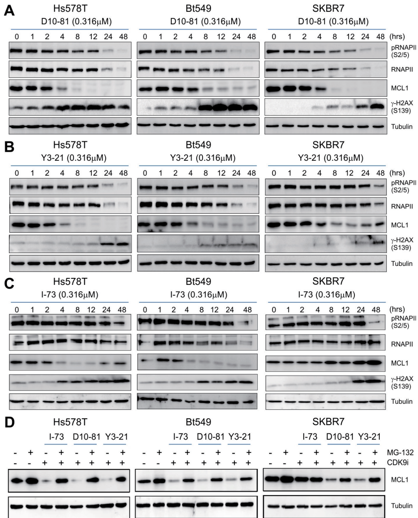
Figure 5. Kinetics of P-TEFb complex inhibition, MCL-1 degradation, and induction of DNA damage in TNBC cells. Effect of D10-81 (A), Y3-21 (B) and I-73 (C) on CDK9-mediated RNAPII phosphorylation, MCL-1 levels and DNA damage marker \gamma -H2AX (S139) in a time course in representative Hs578T, BT549 and SKBR7 cells. Cells were treated with vehicle control (DMSO) or inhibitor (0.316 \mu M) for the indicated duration. (D) Proteasome dependence of CDK inhibitor-mediated MCL1 depletion in TNBC cell lines Hs578T, BT549 and SKBR7. Cells were pre-treated with proteasome inhibitor (MG-132; 10 \mu M) for 2 hours before being treated with vehicle (DMSO) or I-73, D10-81 or Y3-21 (0.316 \mu M) for 6 hours.
