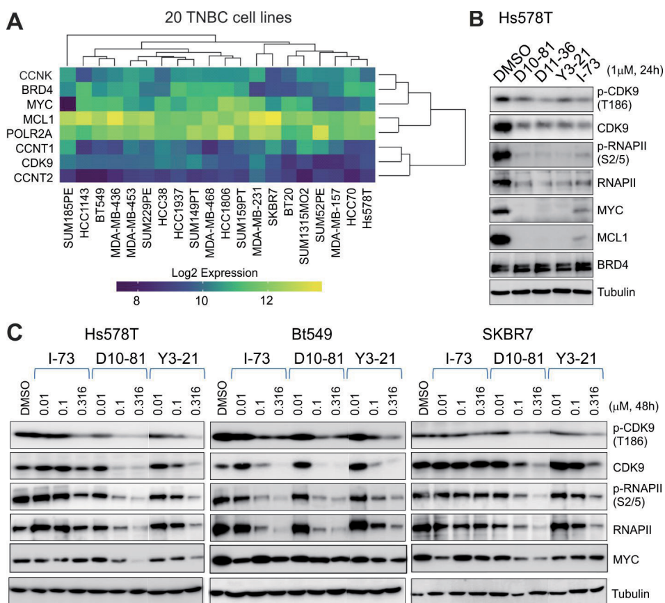
Figure 3. Targeting CDK9 inhibits P-TEFb-mediated transcriptional signaling transduction in TNBC cells. (A) Expression of P-TEFb complex members and associated components in various TNBC cell lines, as established by RNA-Seq analysis at Log2 expression levels. (B) Effect of CDK9 inhibitors D10-81, D11-36, Y3-21 and I-73 on P-TEFb activity and downstream targets in Hs578T cells. Cells were treated with inhibitors at 1μM for 24h. JQ1, BRD4 inhibitor. (C) Impact of I-73, D10-81 and Y3-21 on P-TEFb activity and downstream targets in representative Hs578T, BT549, and SKBR7 TNBC cells 48h post-exposure to each inhibitor in dose range (0.01, 0.1 or 0.316 μM),
