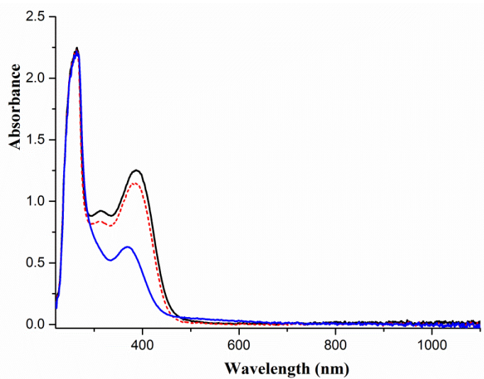
Figure AI.23. UV-vis spectra recorded upon addition of 2 equiv. (red dotted line), and 4 equiv. (blue line) AgBF 4 to a solution of the compound 1 Fe . The spectra were recorded in at a concentration of 2 mM [Fe] with a transmission dip probe path length of 2.2 mm.
