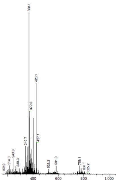
Figure AIII.13. ESI-MS spectrum of the reaction mixture of 3 with H 2 O 2 after the first one hour. ESI-MS found (calcd) for [Co III (L 1 SO)Cl] + m/z 368.1 (368.0); [Co III (L 1 SO 2 )Cl + MeCN] + m/z 425.1 (425.0).
