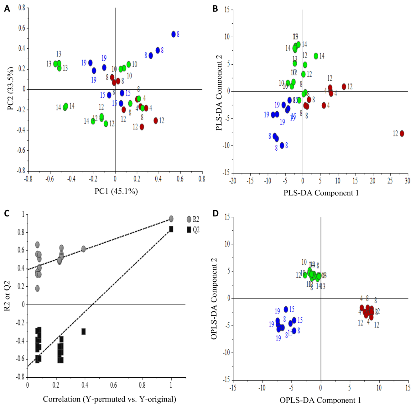
Fig. 4 Multivariate data analyses of Catharanthus roseus cells constitutively overexpressing CrGES (red color), \Delta pl CrGES (blue color), and the control C. roseus cells transformed with empty vector (green color). Principal component analysis (PCA) score plot (a), partial least squares-discriminant analysis (PLS-DA) score plot (b),
