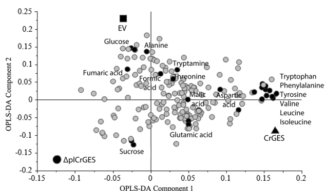
Fig. 5 Loading plot of orthogonal projection to latent structures-discriminant analysis (OPLS-DA) of Catharanthus roseus cells constitutively overexpressing CrGES , \Delta pICrGES , and the control C. roseus cells transformed with empty vector (EV). Variables X (metabolite signals) located closely to variable Y ( CrGES , \Delta pICrGES , EV) contributes to the separation of the samples. The grey circles are the metabolites signals and the dark black circles are the signals of identified metabolites listed in the Table 1
