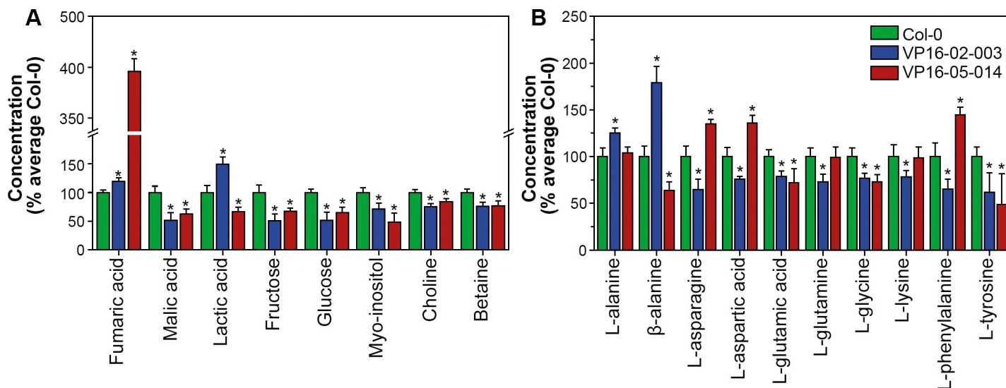
Fig 4. Metabolic alterations in the leaf of Arabidopsis thaliana VP16-02-003 and VP16-05-014 plants as compared to Col-0 plants grown in a 12h-light/12h-dark regime by ^1\text{H} HR-MAS NMR. (A) Relative levels of organic acids, sugars, sugar alcohol, precursor of cell wall components and organic osmolyte in leaves of VP16-02-003 and VP16-05-014 plants in comparison to the level in Col-0. (B) Relative levels of free amino acids in leaves of VP16-02-003 and VP16-05-014 plants in comparison to Col-0. Concentrations are represented by the mean \pm SEM averaged over n = 8 samples. The asterisks (*) indicate significant differences between concentrations for Col-0 and mutants, calculated with Student's t -test ( p < 0.05 ).
