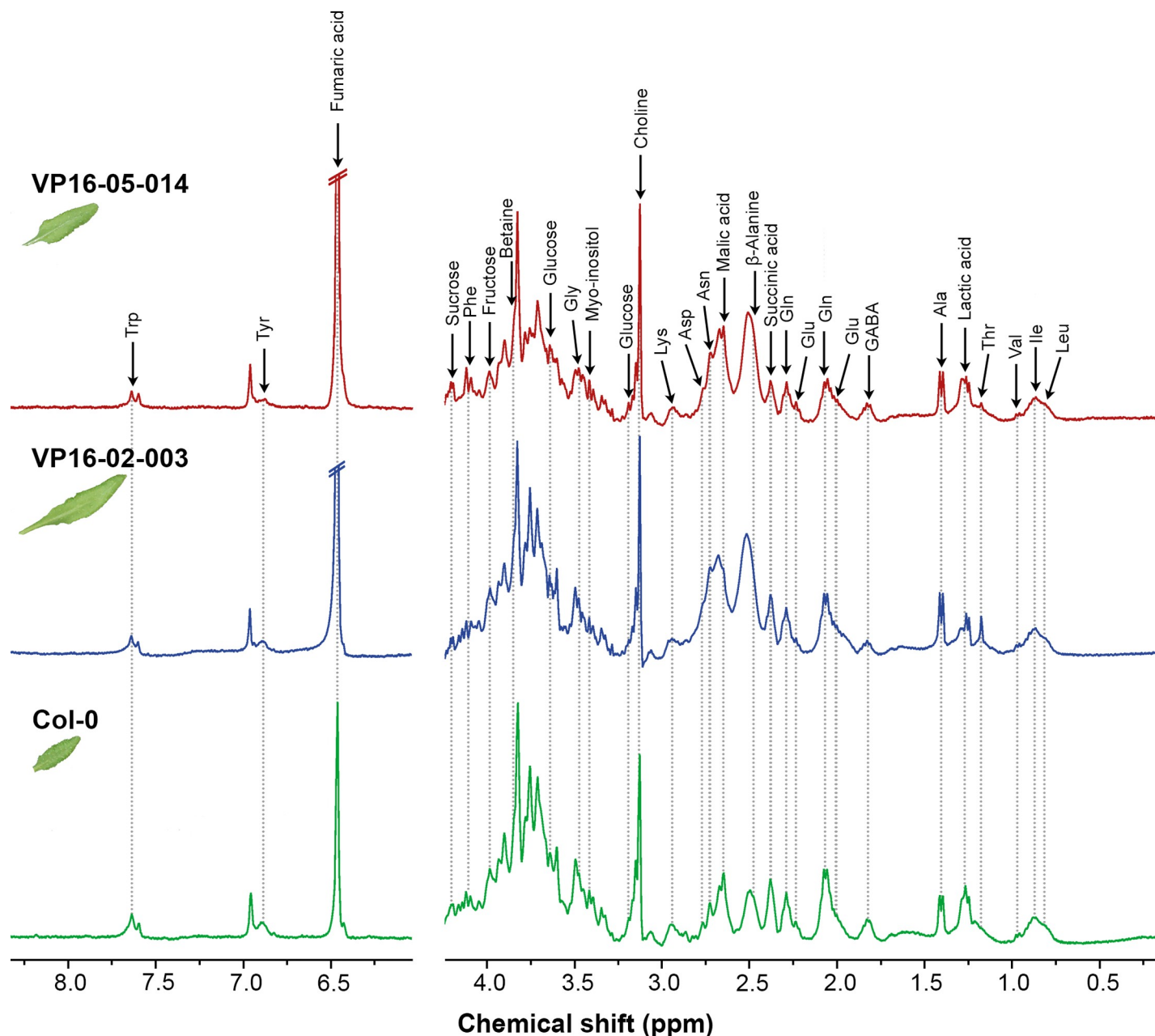
Fig 2. Representative one-dimensional ^1\text{H} HR-MAS NMR spectra collected from intact leaves of Arabidopsis thaliana Col-0 (bottom panels), VP16-02-003 (middle panels) and VP16-05-014 (top panels) grown in a 12h-light/12h-dark regime. The intact leaves were harvested 28 dpg at t = 6 hours (6 hours after the beginning of the light period) for the measurement. The signals from the assigned metabolites have been shown in the spectra (see S2 Table for assignment).
