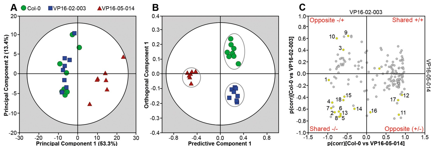
Fig 3. Multivariate analysis of ^1\text{H} HR-MAS NMR metabolic data collected from Arabidopsis thaliana Col-0 (●), VP16-02-003 (■) and VP16-05-014 (▲). (A) PCA score plot with R^2X = 0.761 and Q^2 = 0.611 . The dark circle shows the 95% confidence interval using Hotelling T^2 statistics. (B) OPLS-DA score plot with R^2X = 0.849 , R^2Y = 0.942 , Q^2 = 0.603 , which indicates separation between the Col-0, VP16-02-003 and VP16-05-014 Arabidopsis plants based on their metabolic profile. The dark circle represents the Hotelling T^2 interval with 95% confidence. (C) SUS plot represents biomarkers responsible for the separation in the score plot. 1. Fumaric acid; 2. Malic acid; 3. Lactic acid; 4. Fructose; 5. Glucose; 6. Myo-inositol; 7. Choline; 8. Betaine; 9. L-alanine; 10. \beta -alanine; 11. L-asparagine; 12. L-aspartic acid; 13. L-glutamic acid; 14. L-glutamine; 15. L-glycine; 16. L-lysine; 17. L-phenylalanine; 18. L-tyrosine.
