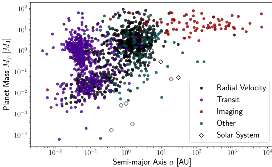
Figure 1.1: Planet mass versus orbital semi-major axis for all planets discovered to date. Extrasolar planets are marked with circles and coloured according to the method used in the detection of the exoplanet. The large diamonds indicate the solar system planets.
