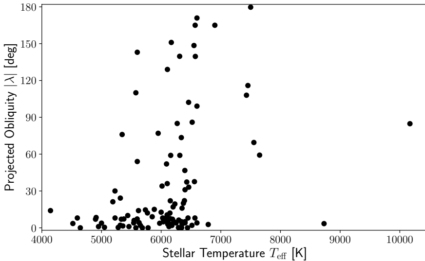
Figure 1.2: Obliquity versus stellar effective temperature for exoplanets. At T_{\text{eff}} \lesssim 6250 K the obliquities are close to 0^\circ as expected from planet formation theories. At higher temperatures the distribution is more random, suggesting some process modifies the alignment during the formation or evolution of planets around hot stars.
