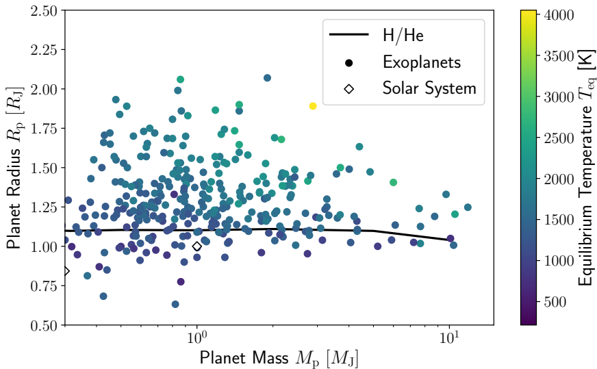
Figure 1.3: Planet mass versus planet radius, hot Jupiters are indicated by circles and solar system planets by the white diamonds. The hot Jupiters are coloured by their equilibrium temperature. The solid line, taken from Baraffe et al. (2008), indicates the mass-radius relation for a 3 Gyr year old H/He gas giant planet at 0.045 AU from the Sun.
