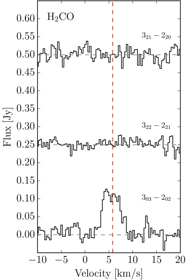
Figure 2.1: Disk-integrated H 2 CO spectra using a 5.6'' radius circular aperture. H 2 CO 3_{03} - 2_{02} , H 2 CO 3_{22} - 2_{21} , and H 2 CO 3_{21} - 2_{20} are at y-offsets of 0, 0.25, and 0.5 Jy, respectively, shown in dashed gray lines. The vertical dashed red line shows the systemic velocity. The spectra are Hanning smoothed to 0.336 km s -1 channels.
