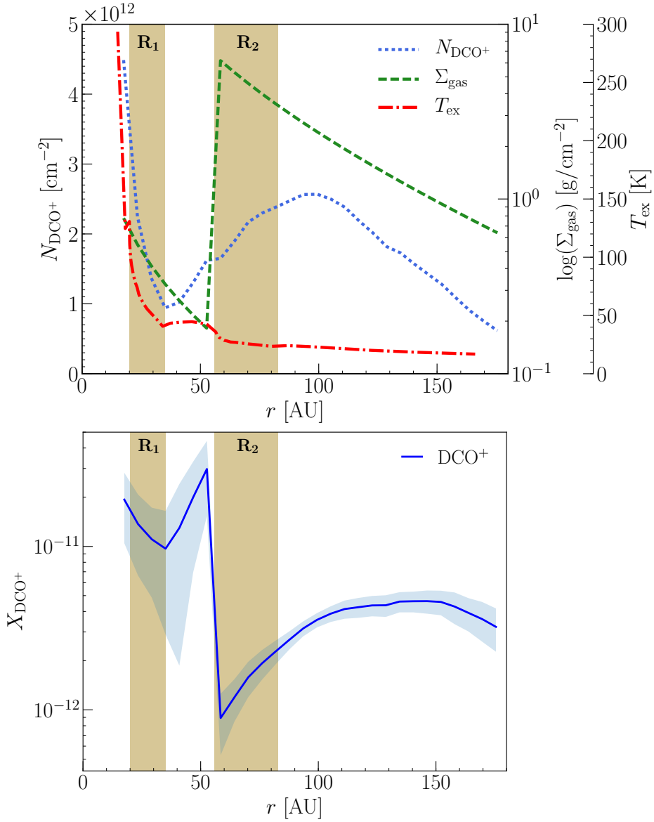
Figure 4.3: One-dimensional, radial structure in the HD 169142 disk. Vertical brown shaded regions represent the dust rings. (Top) The \text{DCO}^+ radial column density (dotted blue) calculated from Equation 4.1 using the \text{DCO}^+ the radial intensity profile (see Figure 4.2) and the midplane gas temperature of the optimized DALI model (dot-dash red) as the T_{\text{ex}} profile. The gas surface density profile (dashed green) was used to derive the \text{DCO}^+ radial abundance. (Bottom) Radial abundance structure of \text{DCO}^+ with respect to \text{H}_2 . The blue shaded region represents 1\sigma errors on the abundance.
