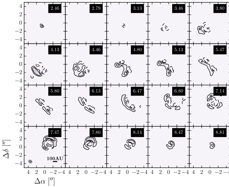
Figure 2.14: \text{C}^{18}\text{O} 2 – 1 residual (data – model) channel maps. Black contours mark 4.2 \times 10^{-3} (1\sigma) \times [5, 10, 20] \text{ Jy beam}^{-1} . Dashed contours are negative at the same intervals. Synthesized beam and AU scale are shown in the lower left panel.
