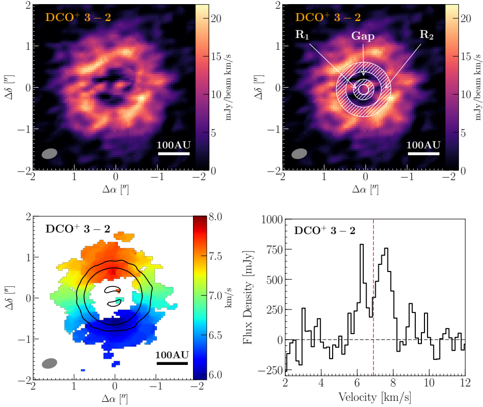
Figure 4.1: (Top left) Integrated intensity map of the DCO + J = 3 - 2 line from 5.4 – 8.8 km s -1 after applying a Keplerian mask to the image cube. The synthesized beam and AU scale are shown in the lower corners. (Top right) DCO + J = 3 - 2 integrated intensity map overlaid with white marking the model inner dust cavity, the inner dust ring (R 1 , hatched), the dust gap, and the outer dust ring (R 2 , hatched). The synthesized beam and AU scale are shown in the lower corners. (Bottom left) Velocity-weighted coordinate map of the DCO + J = 3 - 2 line, clipped at 3.5\sigma . Solid black contours show the 233 GHz/1.3 mm emission at 7.0 \times 10^{-5} Jy beam -1 ( 1\sigma ) \times [5, 50, 200]. The synthesized beam and AU scale are shown in the lower corners. (Bottom right) Disk-integrated spectrum of the DCO + J = 3 - 2 line before Keplerian masking, Hanning smoothed to 0.17 km s -1 channels. The horizontal dashed black line indicates the continuum-subtracted spectral baseline. The vertical red line shows the systemic velocity at 6.9 km s -1 .
