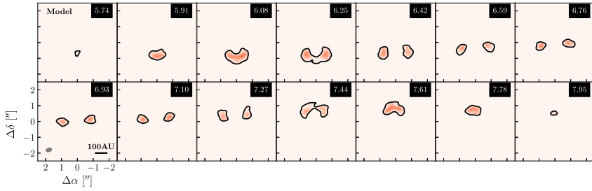
Figure 4.9: DCO + J = 3 - 2 best-fit model channel maps. Black contours show 5.5 mJy beam -1 ( 1\sigma ) \times [3]. Channel velocity is shown in the upper-right corner. The synthesized beam and AU scale are shown in the lower-left panel.
