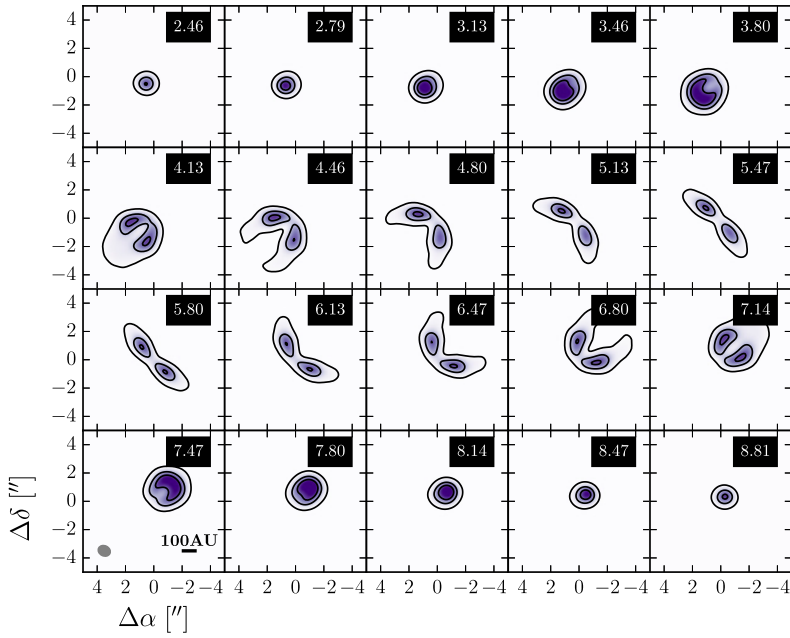
Figure 2.13: C 18 O 2 – 1 best-fit model channel maps. Black contours mark 4.2 \times 10^{-3} ( 1\sigma ) \times [5, 25, 45] Jy beam -1 . Synthesized beam and AU scale are shown in the lower left panel.
