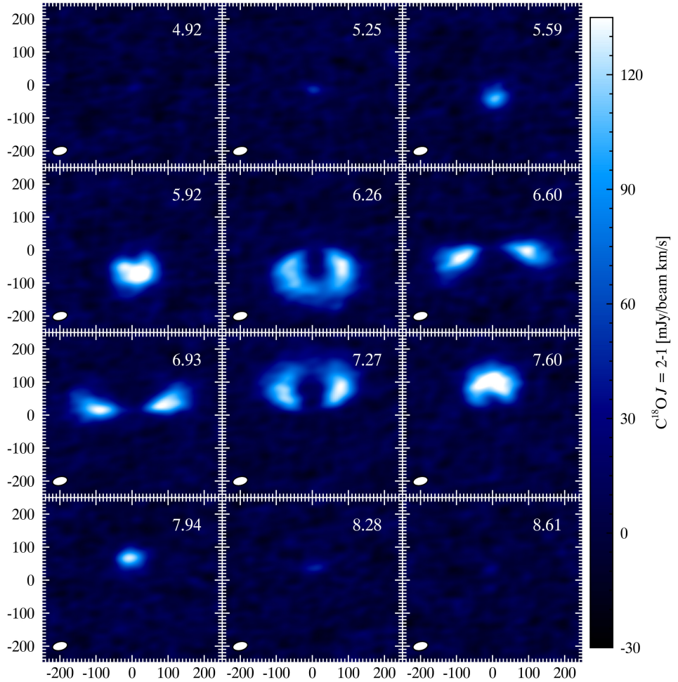
Figure 3.10: ALMA channel maps of \text{C}^{18}\text{O } J = 2 - 1 .
