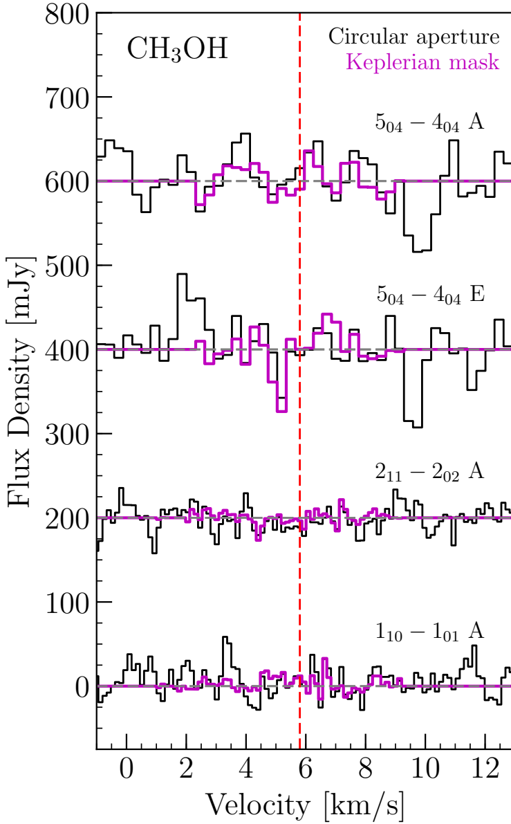
Figure 5.1: Spectra at the expected velocity of \text{CH}_3\text{OH} line emission in the HD 163296 disk showing non-detections from aperture-masked image cubes using an 8" diameter circular aperture (black) and Keplerian-masked image cubes (magenta). The two bottom spectra are observed in band 7 in 0.139 \text{ km s}^{-1} channels while the two top spectra are in band 6 in 0.303 \text{ km s}^{-1} channels. The horizontal gray dashed line represents the spectrum baseline, which is offset by 200 mJy for each line. The vertical red dashed line shows the systemic velocity at 5.8 \text{ km s}^{-1} (Qi et al. 2011).
