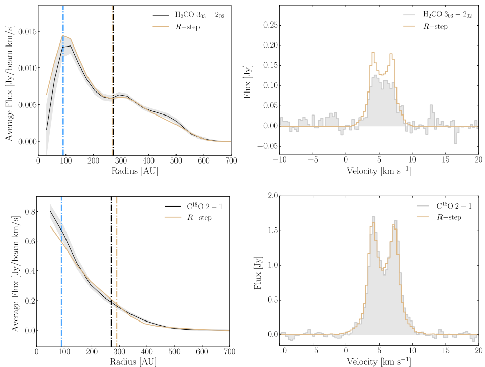
Figure 2.7: Radial intensity and spectra of observed \text{H}_2\text{CO } 3_{03}-2_{02} and \text{C}^{18}\text{O } 2-1 versus the best-fit models. (Left) Radial intensity curves from azimuthally-averaged elliptical annuli projected to i = 44^\circ , P.A. = 133^\circ . HD 163296 data is shown in black, best fits for \text{H}_2\text{CO} and \text{C}^{18}\text{O} are in gold. The vertical dashed lines indicate the CO snow line (blue dash) from Qi et al. (2015), the 5\sigma outer radius of the 1.3 mm grains (black dash), and the change-over radii, R_c , for the best-fit radial step-abundance models (gold dash). \text{H}_2\text{CO} profiles are taken from integrated intensity maps after applying a Keplerian mask. (Right) Disk-integrated spectra. HD 163296 data is shown in filled gray. \text{H}_2\text{CO} spectra are Hanning smoothed to 0.336 \text{ km}^{-1} channels.
