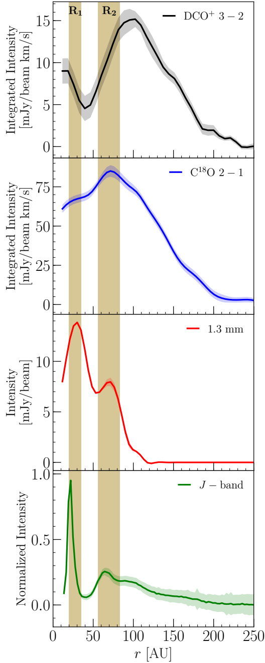
Figure 4.2: Azimuthally averaged radial intensity profiles of \text{DCO}^+ (top), \text{C}^{18}\text{O} (top middle), the 1.3 millimeter continuum (bottom middle), and the J -band ( \sim 1.2 \mu\text{m} ) polarized light (bottom). Shaded regions represent 1\sigma errors on the intensity. Vertical brown shaded regions represent the dust rings.
