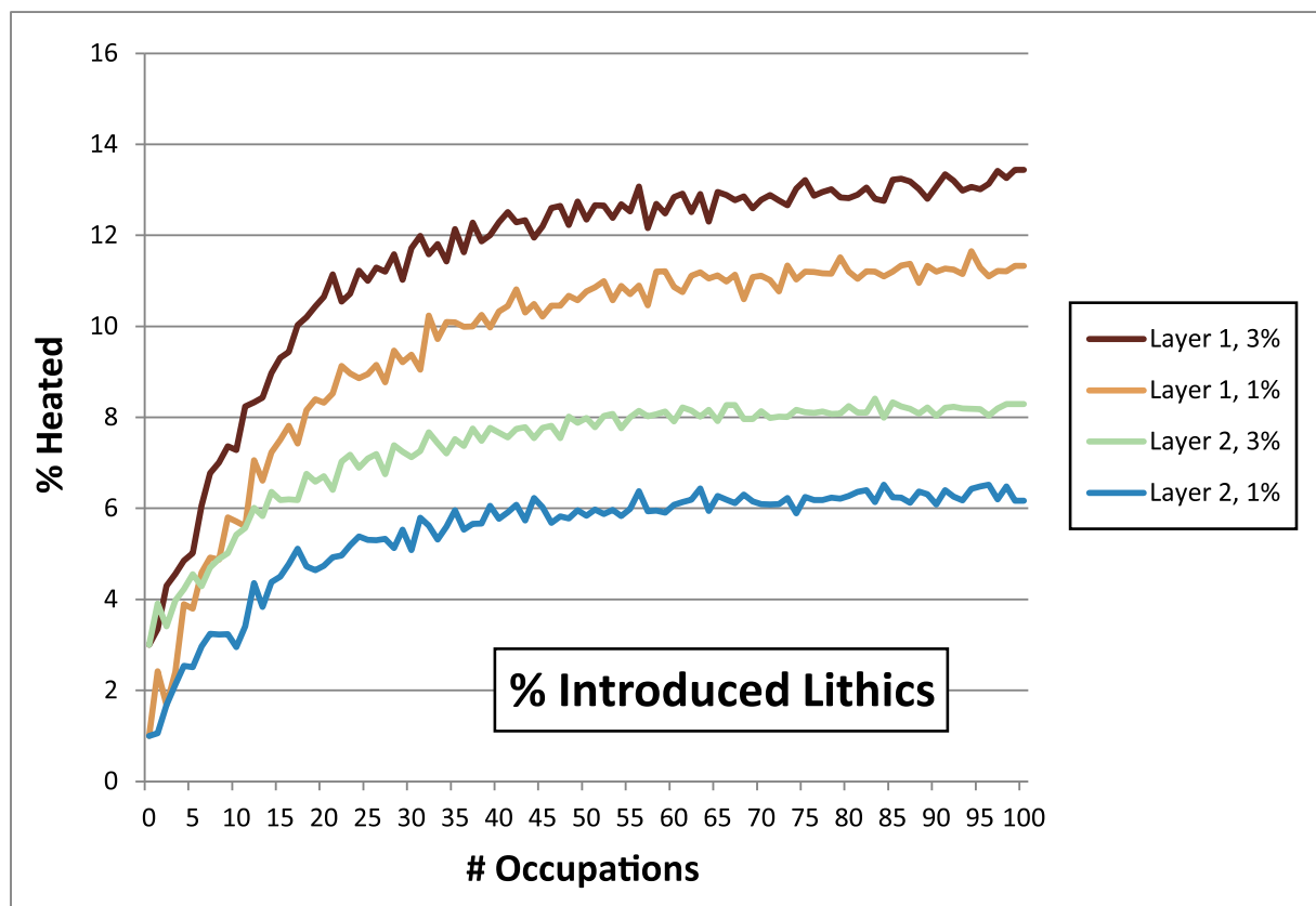
Fig 13. Chart demonstrating the effects of increasing the number of lithic artefacts introduced directly into a hearth (i.e. introduced lithics, see Section 2.1) from 1% to 3%. Parameters: Fires Random/Lithic Scatters Random (FR/LSR), 1 fire, fire size 1, 4 lithic scatters, 5% TB. Changing this percentage only appears to affect the final percentages by around the same number.
