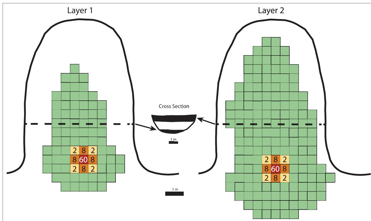
Fig 2. Diagrams depicting the layouts of the hypothetical cave and occupation layers utilized in the simulations. The grid cells delimit the extents of Layer 1 (left: 40 m 2 in 80–50-cm 2 units) and Layer 2 (right: 80 m 2 or 160–50-cm 2 units). The red, orange and yellow grid cells indicate the relative distribution of lithic fragments within individual lithic scatters, the numbers expressing the percentage of lithic artefacts deposited in each grid cell. Lithic artefacts are absent in green grid cells. The dashed lines delineate the stratigraphic cross-section of the cave deposits (center), with the shaded portions corresponding to Layer 1 (lower) and Layer 2 (upper).
