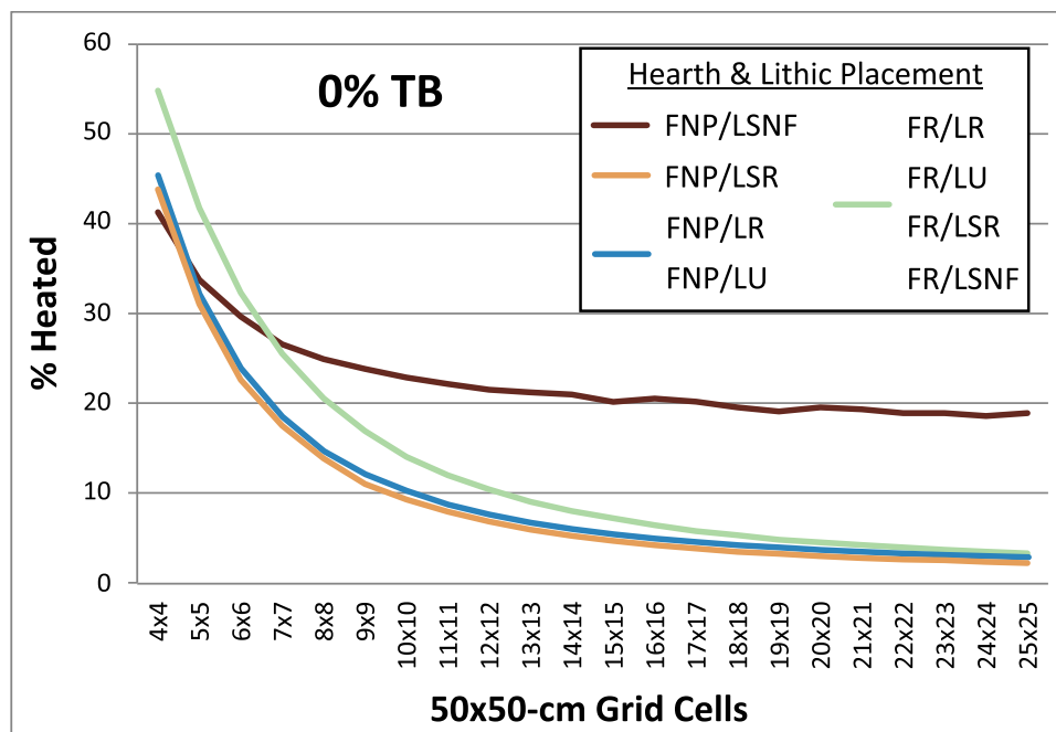
Fig 4. Chart comparing occupation surface size and various fire and lithic scatter placement scenarios. Parameters: 1 fire, fire size 1, 4 lithic scatters, 30 occupations, 1% introduced lithics. Given the near identical results obtained for simulations using the FNP/LR and FNP/LU settings (blue), as well as for all simulations using the FR setting (green), for the sake of clarity these are shown here as single curves. FNP = Fire near previous, FR = Fires random, LSNF = Lithic scatters near fire, LSR = Lithics scatters random, LR = Lithics random, LU = Lithics uniform, TB = Thermal buffering.
