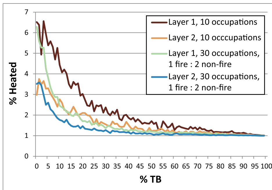
Fig 12. Chart comparing a layer with hearths every third occupation (30 occupations total) with a layer with 10 occupations and fire in every occupation. Parameters: Fires Random/Lithic Scatters Random (FR/LSR), 1 fire, fire size 1, 4 lithic scatters, 0–100% TB, 1% introduced lithics.
