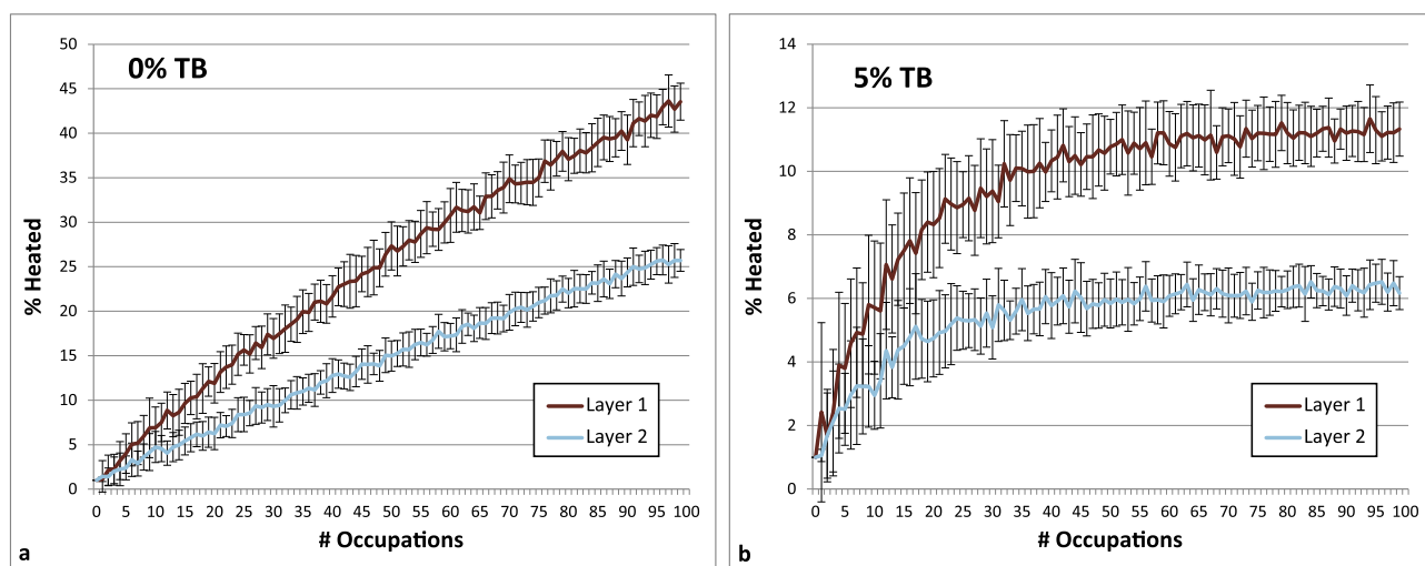
Fig 7. Charts demonstrating how the number of occupations per layer impacts heated lithic percentages for Layer 1 and Layer 2. Parameters: Fires Random/Lithic Scatters Random (FR/LSR), 1 fire, fire size 1, 4 lithic scatters, 0% and 5% TB, 1% introduced lithics.
