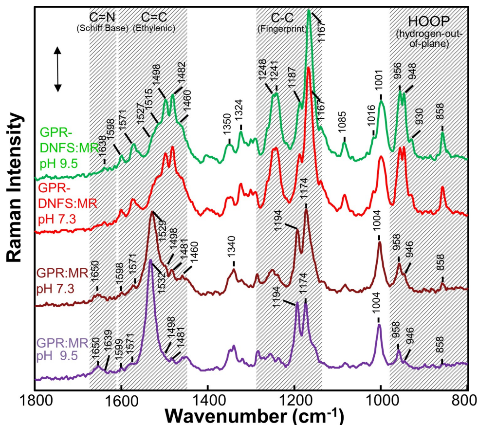
Fig 4. FT-Raman spectra recorded using 1064-nm excitation of GPR:MR and GPR-DNFS:MR at different pHs in reconstituted membrane vesicles. The GPR:MR spectra at the different pHs were scaled using the 1194 \text{cm}^{-1} band and the GPR-DNFS:MR spectra at the different pHs were scaled using the 1167 \text{cm}^{-1} band. Laser power and data acquisition times for each sample were GPR-DNFS:MR pH 7.3 (300 mW, 120 min), GPR-DNFS pH 9.5 (300 mW, 113 min); GPR:MR pH 7.3 (400 mW, 113 min); GPR:MR pH 9.5 (400 mW, 226 min). The scale bar shown is for the GPR-DNFS MR pH 7.3 spectrum and corresponds to 0.005 FT-Raman intensity measured by a Ge detector (see Materials and Methods for additional details).
