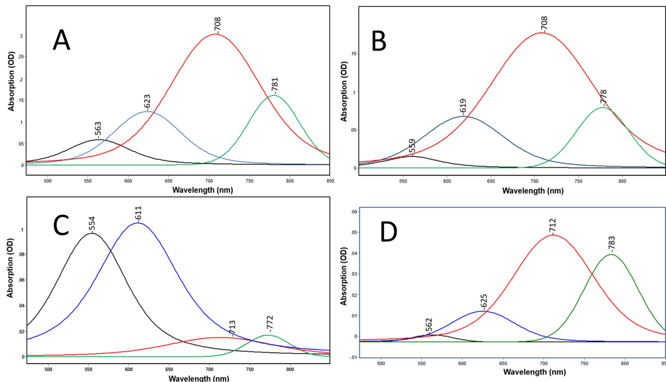
Fig 3. A-D. Curve fitted components of absorption spectra shown in Fig 2 for GPR-DNFS:MR at different pHs. (A) GPR-DNFS:MR at pH 5 in hydrated film; (B) GPR-DNFS:MR at pH 9.5 in hydrated film; and (C) GPR-DNFS:MR at pH 9.5 in aqueous buffer (see Materials and Methods). All spectra are scaled to the largest component peak. Curve fitted components are colored black, blue, red and green from lowest to highest wavelength of component peak maxima. See Materials and Methods for details of curve fitting method.
