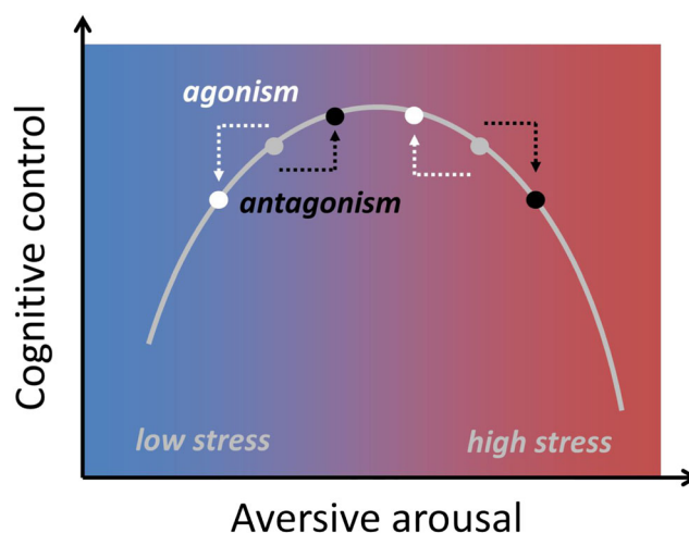
Fig. 5 U-shaped relationship between aversive arousal and cognitive control. Opioids agonist might reduce aversive arousal (white), whereas opioid antagonist might increase it (black). According to this hypothesis, drug effects on cognition depend on the baseline level of aversive arousal, such that an opioid agonist might improve performance in high stress contexts, yet impair performance under low stress.
