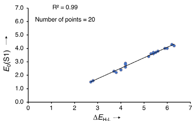
Figure 1. Correlation between HOMO-LUMO gap ( \Delta E_{\text{H-L}} ) of the D- \pi -A molecule and the lowest singlet excitation energy ( E_0(\text{S1}) ), computed at CAMY-B3LYP/TZ2P//BP86/TZ2P. [Color figure can be viewed at wileyonlinelibrary.com]
