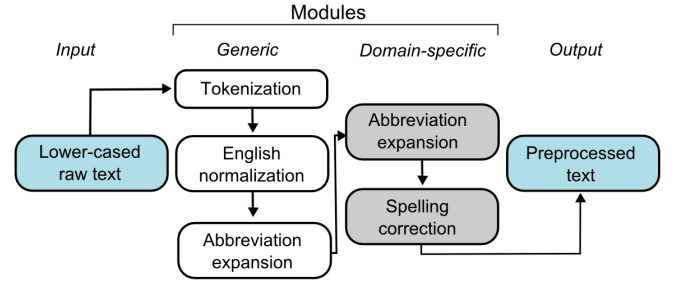
Figure 1: Sequential processing pipeline
