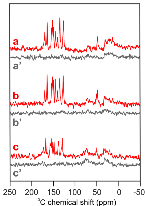
Figure 2. ^{13}\text{C} MAS NMR spectra of selectively 4-ALA ^{13}\text{C} -isotope labeled BBY preparation (a), thylakoid membranes (b) and entire plants (c) of the aquatic plant Spirodella oligorrhiza obtained under continuous illumination (red). Spectra (a'–c') (grey) show the corresponding spectra obtained under dark conditions. All spectra were obtained at a magnetic field of 4.7 T and a temperature of 235 K with a MAS frequency of 8 kHz and a cycle delay of 4 s.
