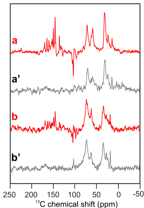
Figure 5. ^{13}\text{C} MAS NMR spectra of natural abundance D1D2 particles of spinach ( a ) and natural abundance core complexes of duckweed ( b ) obtained under continuous illumination (red). Spectra ( a' and b' ) show the corresponding spectra obtained under dark conditions (grey). All spectra were obtained at a magnetic field of 4.7 T and a temperature of 235 K with a MAS frequency of 8 kHz and a cycle delay of 4 s.
