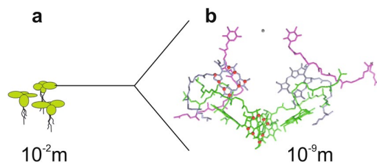
Figure 4. By combining specific ^{13}\text{C} isotope labelling with photo-CIDNP MAS NMR, in the plant of Spirodela oligorrhiza (duckweed, (a)), the red labelled nuclei of the active Chl a and Phe a cofactors (red dots) of the PS2 RC (b) are directly detected without further isolation.
