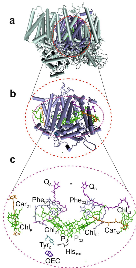
Figure 1. The PS2 core complex (a) is embedded inside the thylakoid membrane (not shown). At the heart of the core complex, the PS2 reaction center (RC) is found (b) and mainly formed by the central D1 and D2 polypeptides. The PS2 RC contains several cofactors (c): two central Chls ( P_{D1} and P_{D2} ), two accessory Chls ( Chl_{D1} and Chl_{D2} ), two pheophytins ( Phe_{D1} and Phe_{D2} ), two quinones ( Q_A and Q_B ), and two peripheral Chls ( Chl_{P1} and Chl_{P2} ). These cofactors are arranged in two symmetrical branches, an active D1 branch (left) and an inactive D2 branch (right). Two \beta -carotenoids ( Car_{D2} and Car_{D1} ) are associated with the PS2 core complex. At the P_{D1} side, a tyrosine residue Tyr_Z is in between P_{D1} and the oxygen evolving system (OEC).
