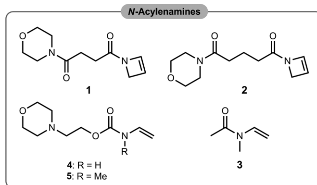
Figure 1. The N -acylazetidines 1 and 2 and N -vinyl derivatives 3–5 .
