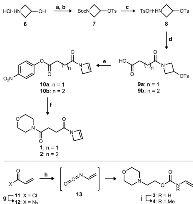
Scheme 1. Synthesis of N -acylazetines 1 , 2 and N -vinylcarbamates 3 , 4 . Reagents and conditions: [a] i: Boc 2 O, TEA, MeOH, 0 °C, 2 h, used crude. [b] TsCl, TEA, DCM, 2 h, 72 % over 2 steps. [c] p TsOH, DCE, reflux, 16 h, 79 %. [d] Succinic- or glutaric anhydride, K 2 CO 3 , MeCN, reflux, 6 h, 50 % 9a , 70 % 9b . [e] KOtBu, DMF, 2 h. ii: bis( p -nitrophenyl)carbonate, 16 h, 80 % 10a , 69 % 10b . [f] morpholine, DCM, 1 h, 84 % 1 , 100 % 2 . [g] NaN 3 , H 2 O/toluene (1:1), 6 h. [h] 2-morpholinoethanol, pyridine, hydroquinone, toluene, 100 °C, 1.5 h, 29 % [j] NaH, THF, MeI, 0 °C, 1.5 h, 75 %.
