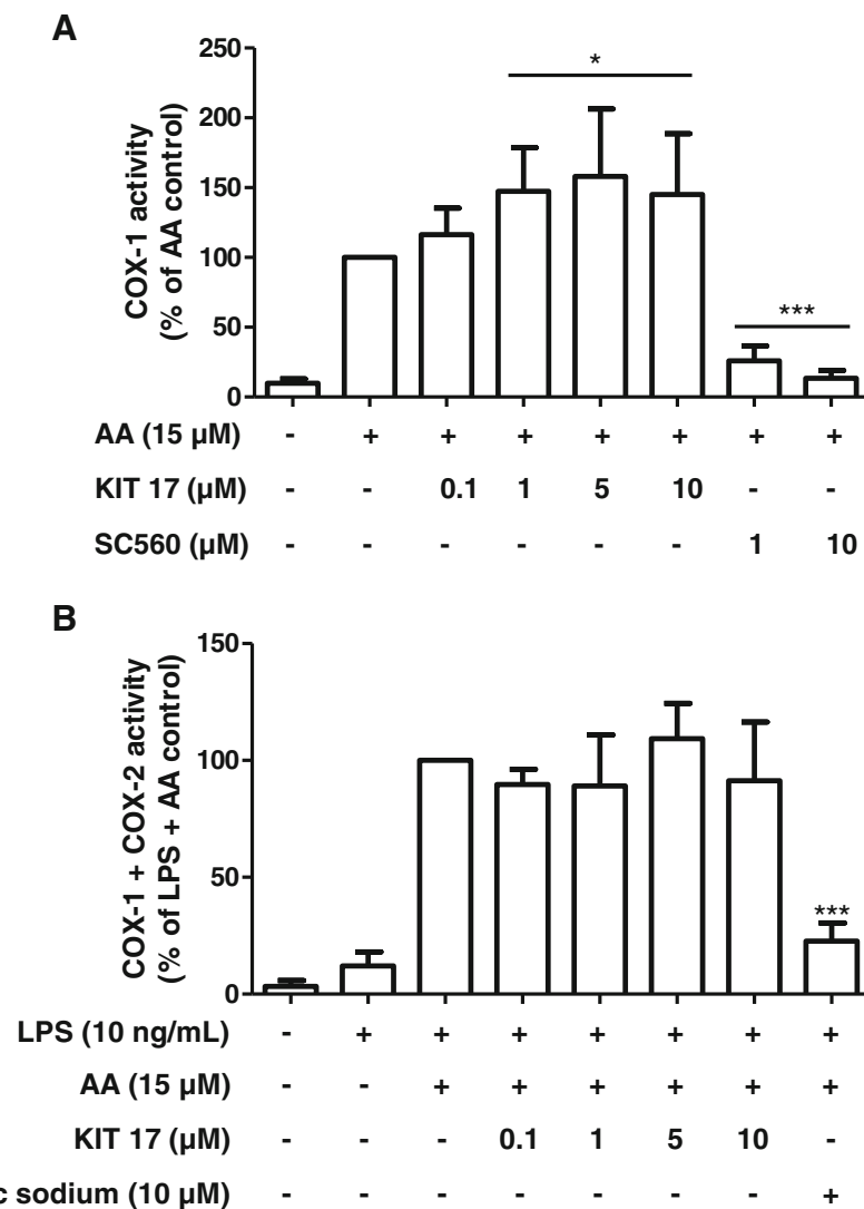
Fig. 7 Effects of KIT 17 on COX-1 (A) and COX-2 (b) enzyme activity in primary microglia cells. a For COX-1 activity assay, cells were treated with different concentrations of KIT 17 for 15 min before addition of 15 \mu M of arachidonic acid. PGE 2 in the supernatants was measured after additional 15 min. b Cells were stimulated for 24 h with LPS (10 ng/mL) and then treated with different concentrations of KIT 17 for 15 min. Then, 15 \mu M of arachidonic acid was added and PGE 2 in the supernatants was measured by enzyme immune assay (EIA). Data are expressed as mean \pm S.E.M. of at least 3 independent experiments. * p < 0.05, ** p < 0.01, and *** p < 0.001 with respect to control (one-way ANOVA followed by the Newman-Keuls post hoc test)
