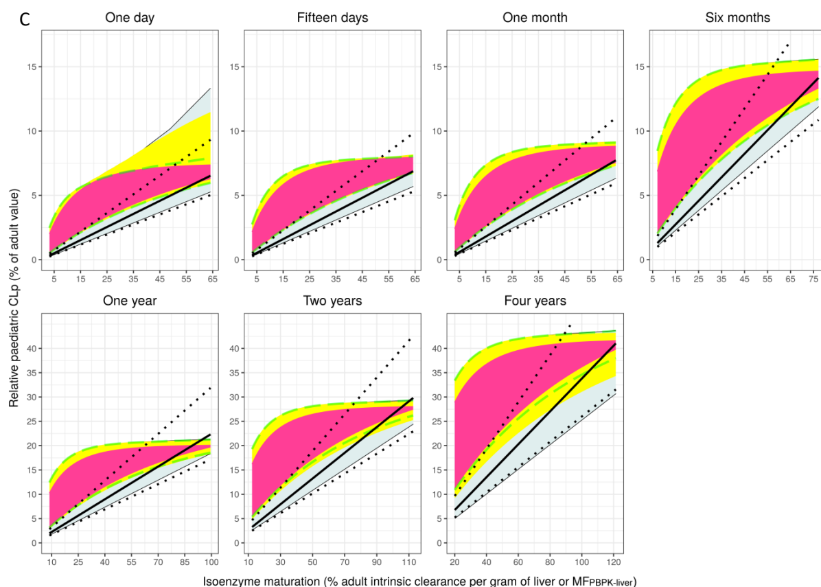
Supplementary Figure 2 Relative paediatric CLp (% of adult value) obtained with AS0.75+MF PBP K-liver scaling (solid black line with \pm 30\% PE as dotted black lines) and 'true' relative paediatric CLp (pink, green and yellow areas) for all hypothetical drugs versus the respective isoenzyme maturation range in the studied typical paediatric individuals. Drugs are categorized by extraction ratio (ER) in adults with low ER ( \leq 0.3 ) in panel A, intermediate ER (0.3-0.7) in panel B, and high ER ( > 0.7 ) in panel C. Different colours represent hypothetical drugs with different properties, with the pink shaded area representing drugs not binding to plasma proteins ( f_u=1 ) that are also in equilibrium between plasma and red blood cells ( K_p=1 ). The area delimited by the two green dashed lines and the yellow shaded area are used to depict drugs that diffuse into red blood cells to different extents and that bind to HSA or AAG, respectively, to different extents (including f_u=1 ). Under the pink area, the pink and yellow areas overlap completely, therefore the combination of pink and yellow areas shows the results for drugs binding to AAG. The blue shaded area depicts all drugs. Note that the scales on the x- and y-axes may be different for different ages.
