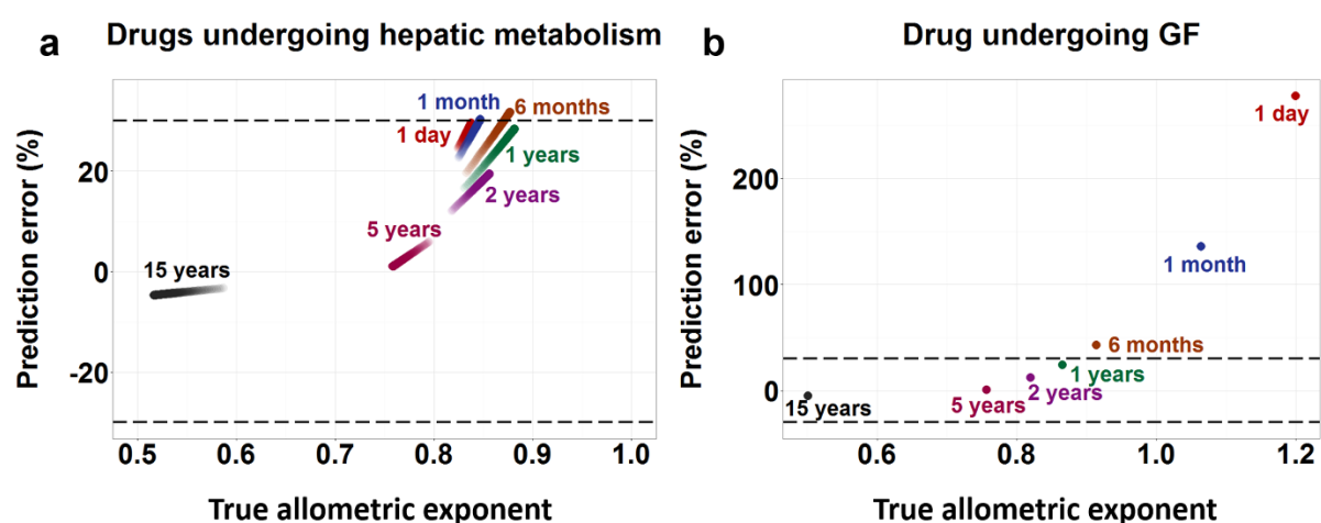
Figure 3 PE of AS0.75 using the fixed allometric exponent of 0.75 in predicting ‘true’ paediatric CL p versus the true allometric exponent for each paediatric age, for drugs undergoing (a) hepatic metabolism or (b) glomerular filtration in scenario 1, where only size-related changes were included in the PBPK-based simulations of ‘true’ paediatric CL p . The values for the different ages are represented with different colours. Colour intensity increases with CL int,mic values of the hypothetical drugs (a). Dotted black lines indicate a PE of \pm 30\% . PE, prediction error; CL p , plasma clearance; PBPK, physiologically-based pharmacokinetic; CL int,mic , unbound microsomal intrinsic clearance.
