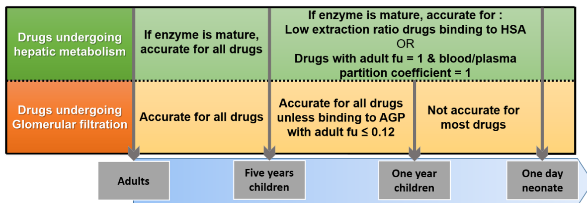
Figure 5 Scenarios for which AS0.75-based paediatric CL p predictions are accurate, based on a PBPK simulation workflow. CL p , plasma clearance; PBPK, physiologically-based pharmacokinetic.
