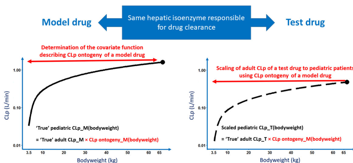
Figure 2 Illustration of between-drug extrapolation of paediatric covariate functions to scale hepatic plasma clearance (CLp) from adults to paediatric patients for drugs eliminated by the same isoenzyme. The black dot in both graphs shows the adult hepatic CLp value for the model drug ('true' adult CLp_M) and the test drug ('true' adult CLp_T). The solid black line represents the change in CLp of the model drug throughout the paediatric age range, which is described by a paediatric covariate function based, in this example, on bodyweight (CLp ontogeny_M (bodyweight)). The dashed black line represents the scaled paediatric CLp predicted for the test drug by between-drug extrapolation of the paediatric covariate function obtained for the model drug (CLp ontogeny_M (bodyweight)). Figure taken from chapter 5 3 .
