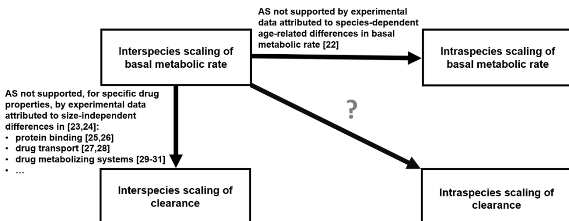
Figure 1 Implicit assumptions underlying the use of AS to scale CL p from adults to children. AS, allometric scaling; CL p , plasma clearance.
