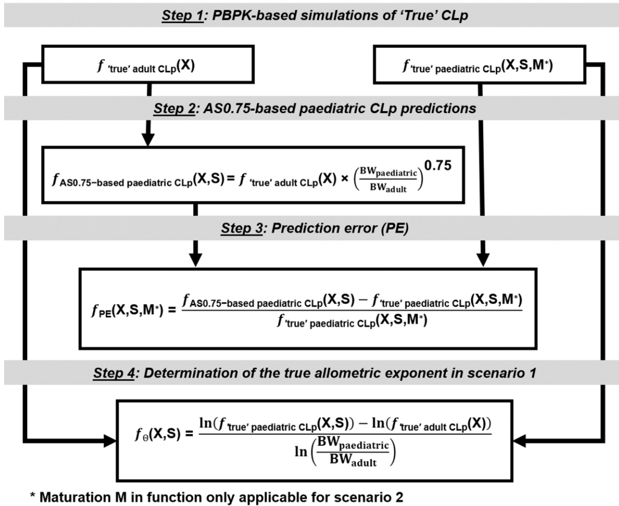
Figure 2 PBPK simulation workflow investigating the predictive performance of AS0.75 on the basis of bodyweight to the power of 0.75, when scaling paediatric CLp from adult CLp values. The simulations include two scenarios: scenario 1 includes size-related changes only, while scenario 2 includes both size-related changes and maturation in the PBPK-based predictions of paediatric CLp. Simulated CLp values are functions of X representing drug-specific properties (i.e., f_u , type of binding plasma protein, CL_{\text{int,mic}} , and K_p ). Paediatric CLp predictions also depend on S representing size-related changes (changes in liver weight, hepatic blood flow, and glomerular filtration) and, in scenario 2, also on M , which represents maturational changes (changes in plasma protein concentration, haematocrit and CL_{\text{int,mic}} ). PBPK, physiologically-based pharmacokinetic; CLp, plasma clearance; f_u , unbound drug fraction in plasma; CL_{\text{int,mic}} , unbound microsomal intrinsic clearance; K_p , blood to plasma partition coefficient.
