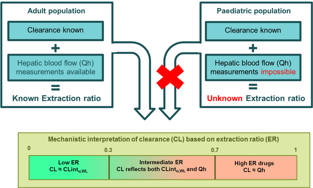
Figure 1 The relationships between extraction ratio (ER), whole liver unbound intrinsic clearance ( CL_{int,u,WL} ) and hepatic blood flow ( Q_h ) for the adult and paediatric population. Without knowing Q_h , the ER of a drug is unknown, making it mathematically impossible to disentangle Q_h and CL_{int,u,WL} from clinical concentration-time data of one drug. CL is the blood clearance of the unbound drug, see equations 1-6.
