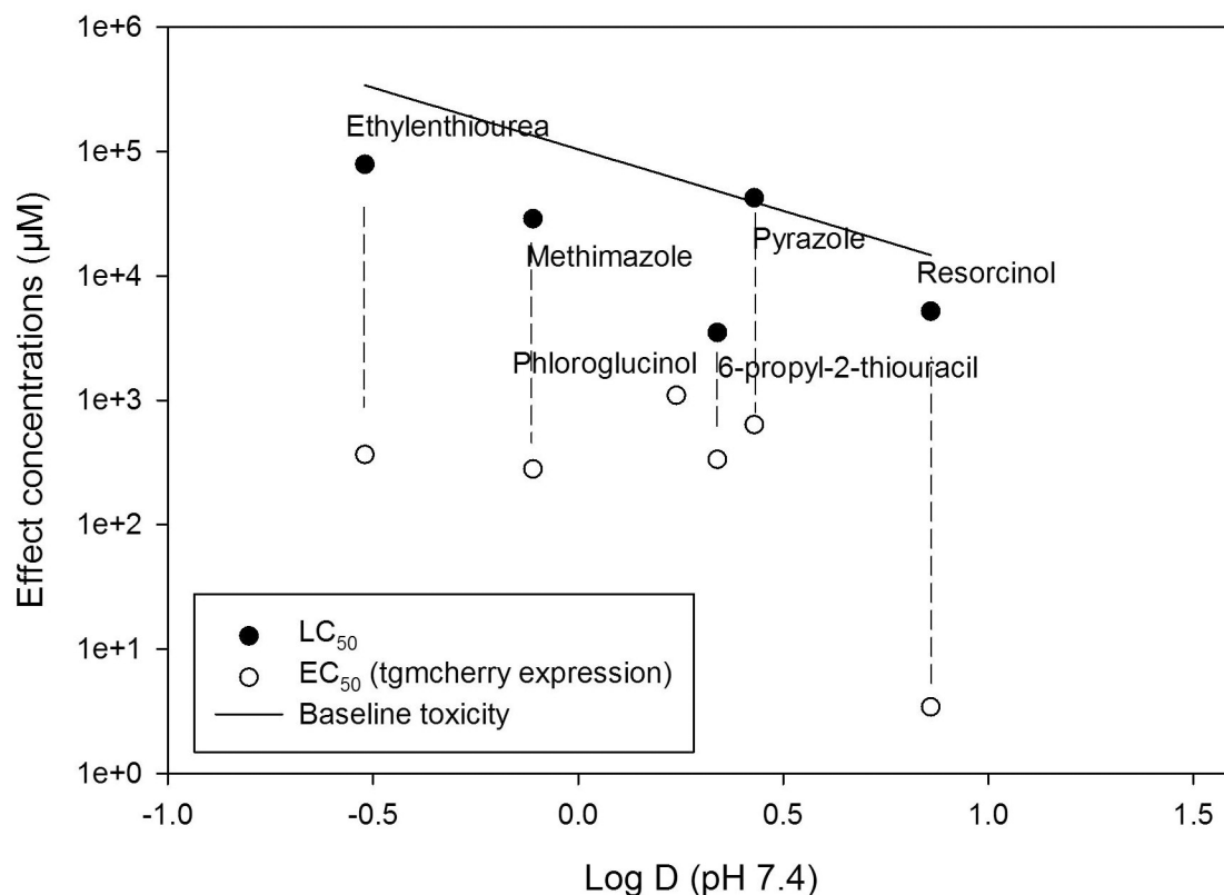
Fig 3. Effect concentrations for tg:mcherry induction and mortality in zebrafish embryo exposed from 48–120 hour post fertilization to known goitrogenic compounds. Effect concentrations are compared to the logD and the baseline toxicity (mortality) to indicate the specificity of the response. Note that the goitrogenic compound potassium perchlorate has not included in this figure given that the use of the logD is not applicable to inorganic compounds. Dashed lines connect the corresponding LC 50 and EC 50 . No mortality was observed for phloroglucinol.
