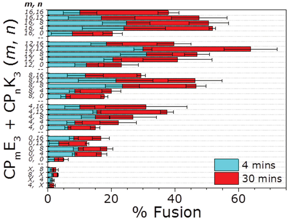
Figure S2. Time resolved rate of fusion (Content mixing) with lipopeptide CP m E or CP n K decorated liposomes as a function of m , n , indicated by an increase in sulforhodamine B emission after 4 and 30 minutes. Left out peptides E or K , ( X ), in negative control experiments are denoted with X , n or m , X . [Total lipid] = 0.1 mM with 1 mol% lipopeptide, in PBS pH 7.4.
