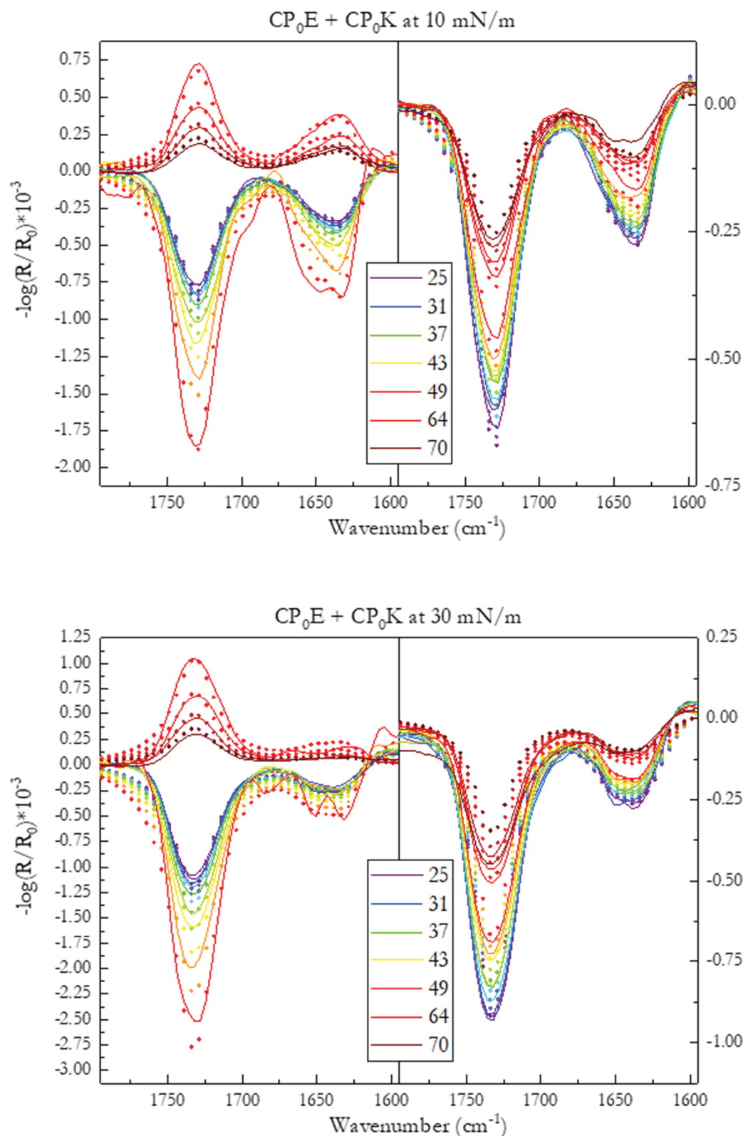
Figure S13. Experimental data of Amide I' absorption bands ( 1600\text{--}1800\text{ cm}^{-1} , lines), and best fits obtained with Matlab (dots) of \text{CP}_0\text{E} and \text{CP}_0\text{K} decorated monolayers at a surface pressure of 10 mN/m and 30 mN/m. Left graphs are angle dependent P-polarized spectra, right graphs are angle dependent S-polarized spectra. Monolayers consists of 4 mol% lipopeptide, D2O PBS pH 7.4.
