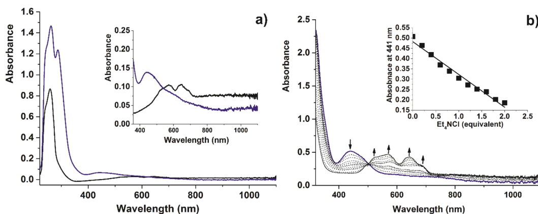
Figure 3. (a) UV–vis spectra of \mathbf{1}_{\text{Co}} (black) and \mathbf{2} (blue). UV–vis spectra were recorded using solutions 1 mM in [\text{Co}] with a transmission dip probe path length of 1.8 mm. The inset shows the UV–vis spectra of compounds recorded of solutions 2 mM in [\text{Co}] . (b) UV–vis spectra recorded upon addition of \text{Et}_4\text{NCl} to a solution of the compound [\text{Co}^{\text{III}}(\text{L}^1\text{S})(\text{MeCN})_2](\text{BF}_4)_2 ( \mathbf{2} ) in acetonitrile. The spectra were recorded in at a concentration of 10 mM [\text{Co}] with a transmission dip probe path length of 2.3 mm. The inset shows the change of absorbance at 441 nm with addition of \text{Et}_4\text{NCl} .
