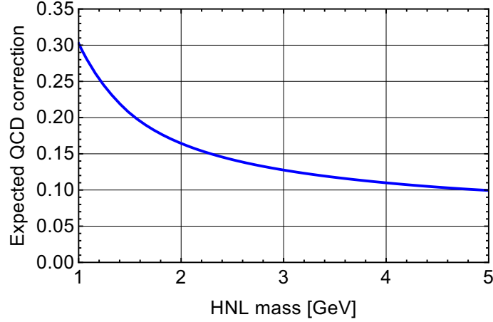
Figure 3.14: The estimate of the QCD corrections for the HNL decay into quark pairs, using the three-loop formula (3.2.11) for \tau -lepton.
