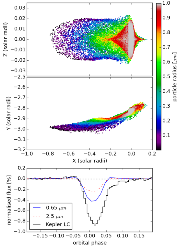
Figure 4.5: Same as a column in Fig. 4.2 except with a mass-loss rate of 3.9 \text{ M}_{\oplus} \text{ Gyr}^{-1} and an intrinsic sublimation rate increased by a factor of three.
