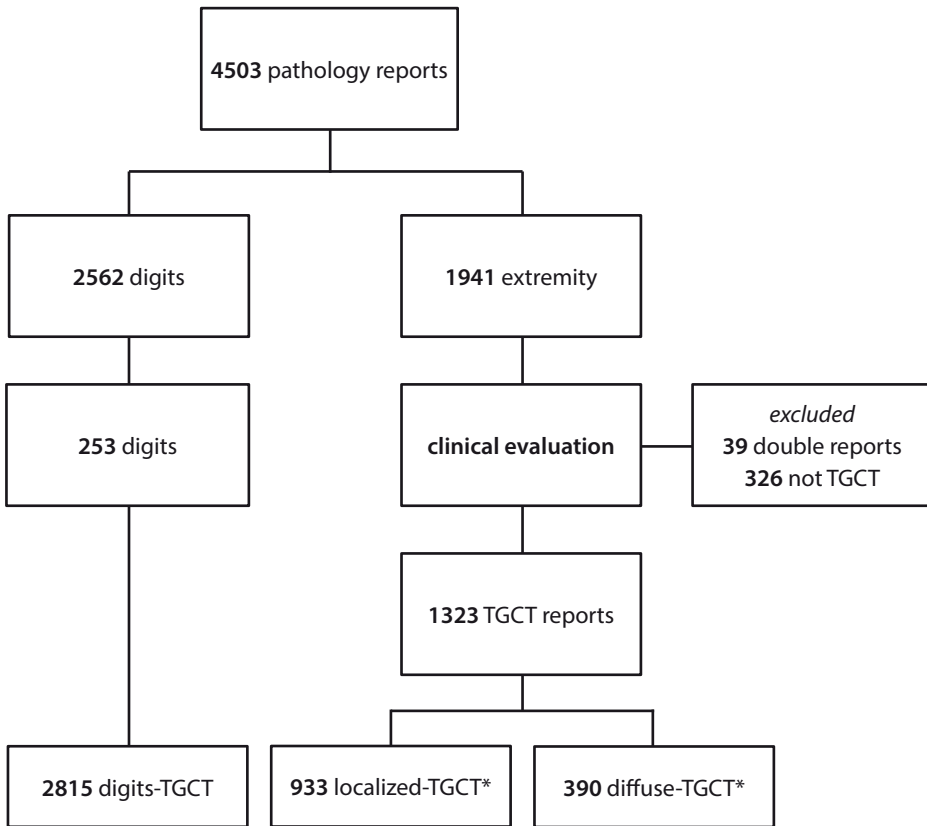
Figure 4 Inclusion flowchart
